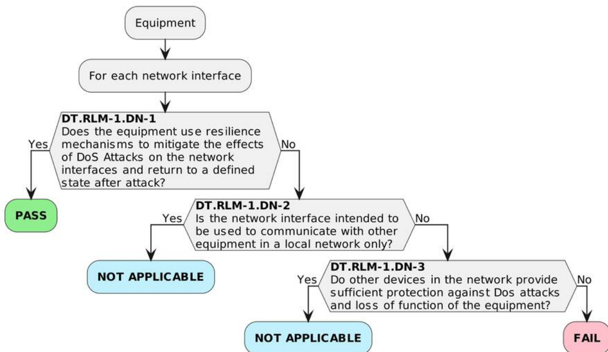
Figure 213 — Decision tree for requirement RLM-1
