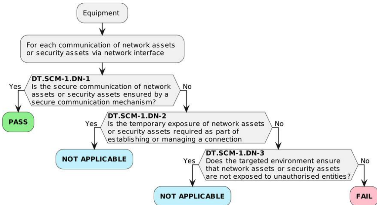
Figure 17 — Decision Tree for requirement SCM-1
