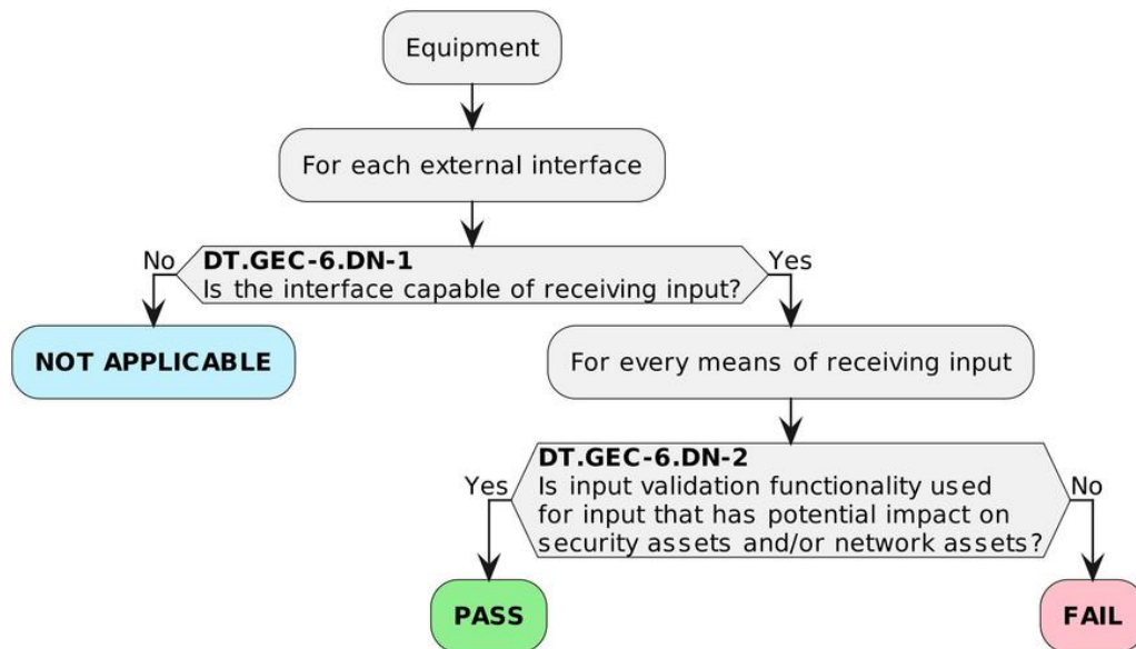
Figure 33 — Decision Tree for requirement CRY-1
