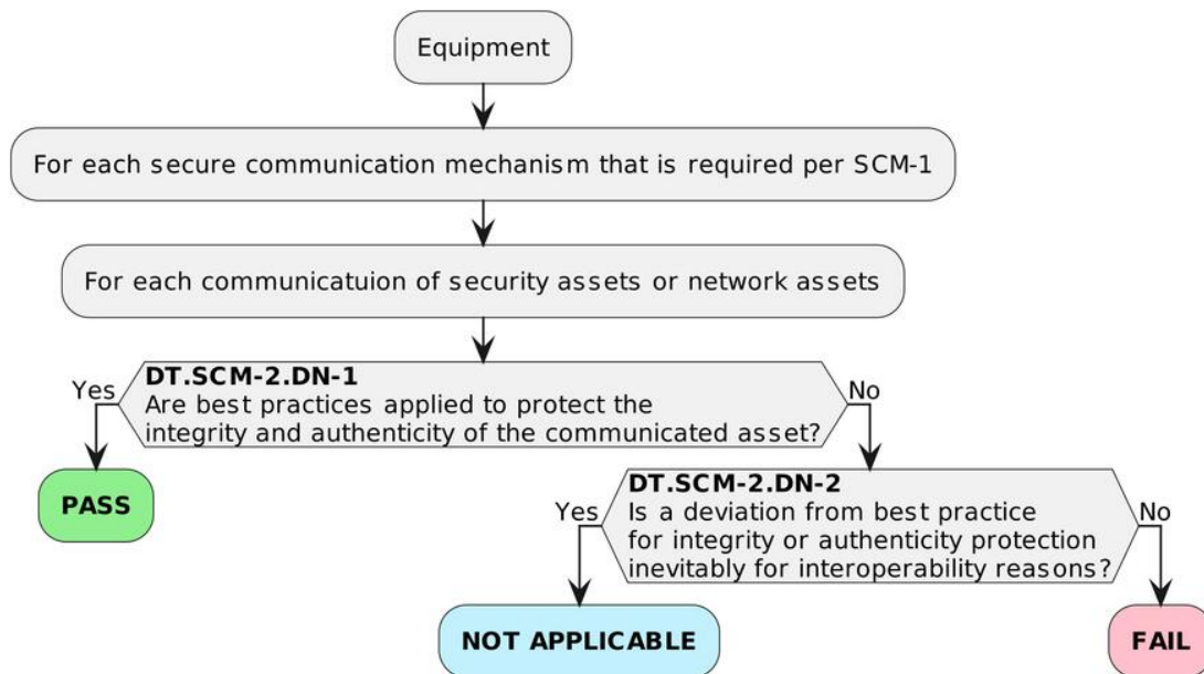
Figure 18 — Decision Tree for requirement SCM-2
