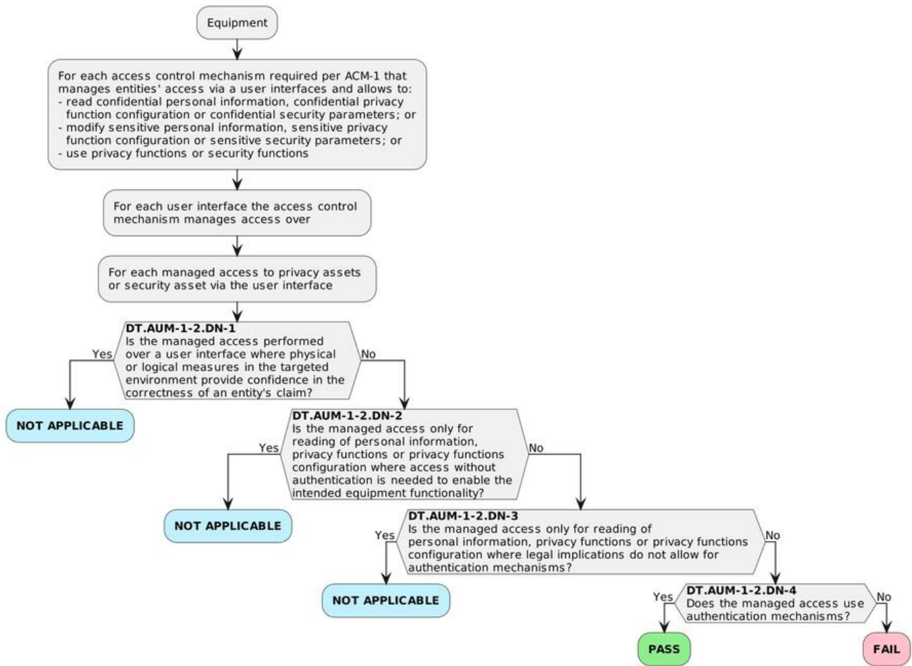
Figure 4 — Decision Tree for requirement AUM-1-2
