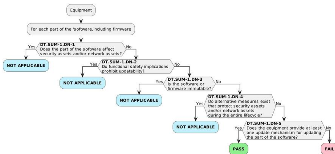
Figure 11 — Decision Tree for requirement SUM-1
