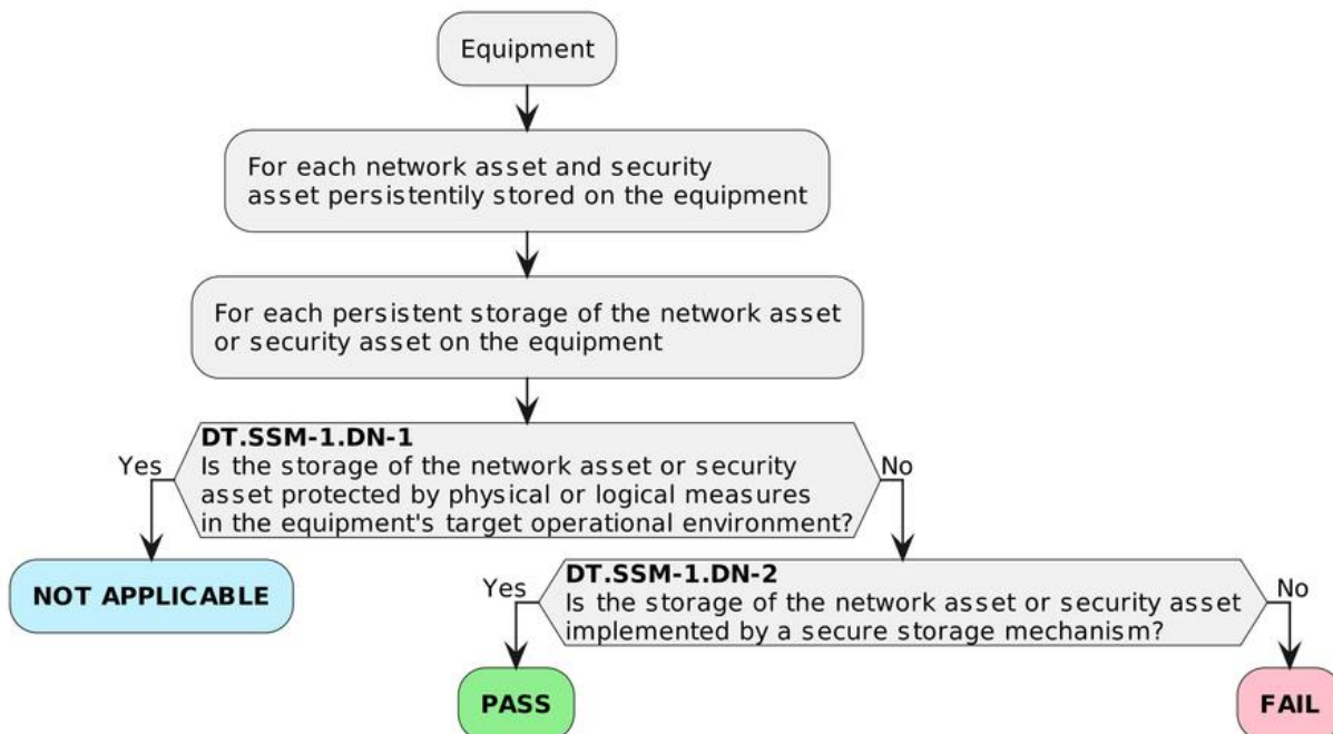
Figure 14 — Decision tree for requirement SSM-1
