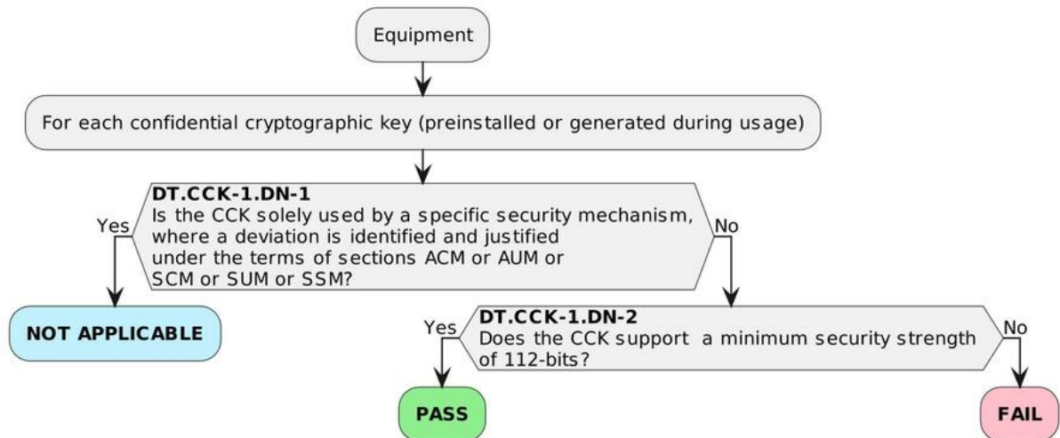
Figure 24 5— Decision Tree for requirement CCK-1
