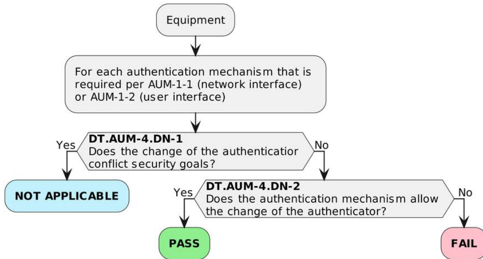
Figure 7 — Decision Tree for requirement AUM-4
