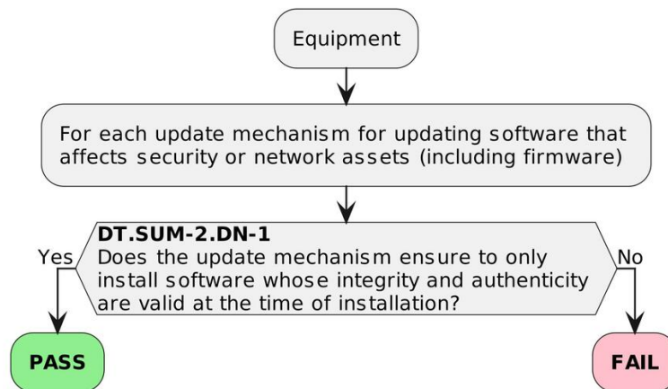
Figure 12 — Decision Tree for requirement SUM-2
