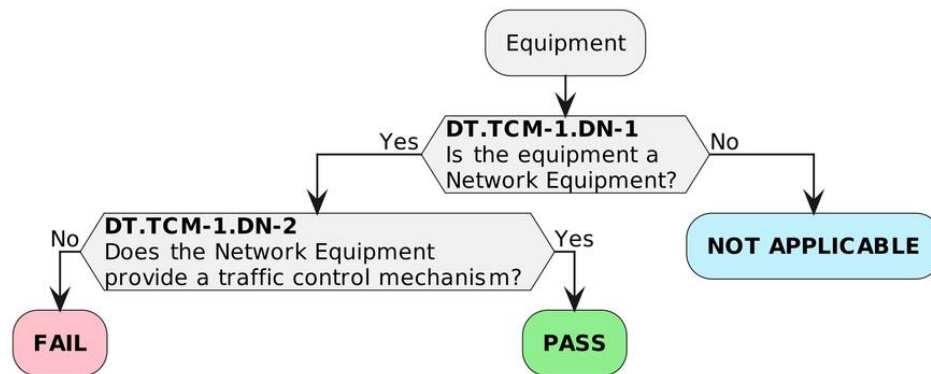
Figure 234 — Decision Tree for requirement TCM-1
