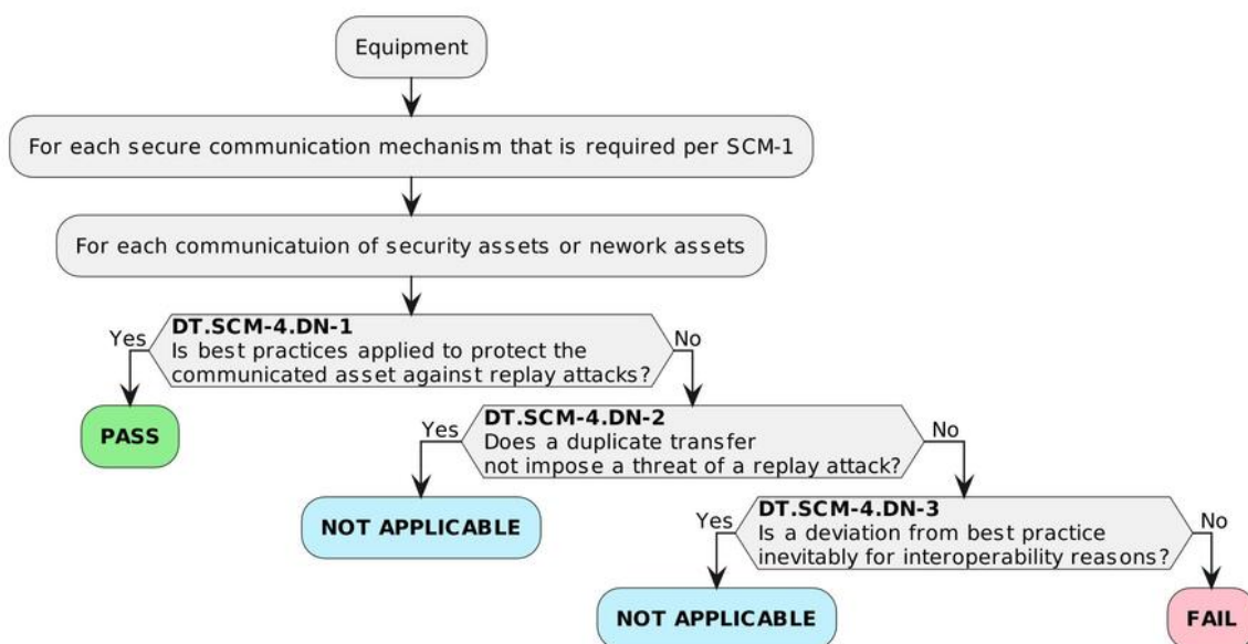
Figure 202 — Decision tree for requirement SCM-4
