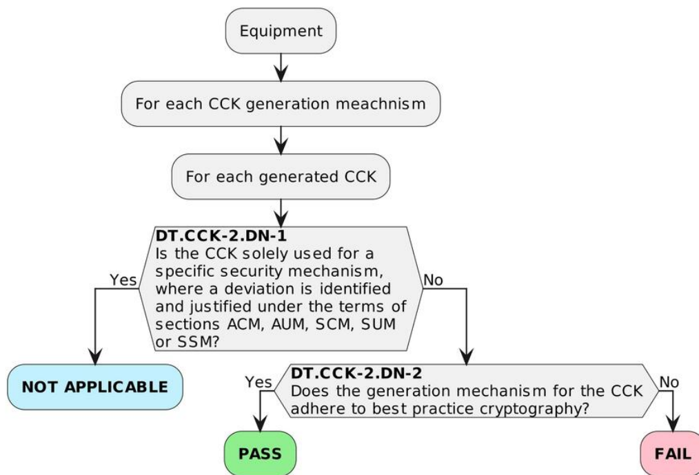
Figure 25— Decision Tree for requirement CCK-2
