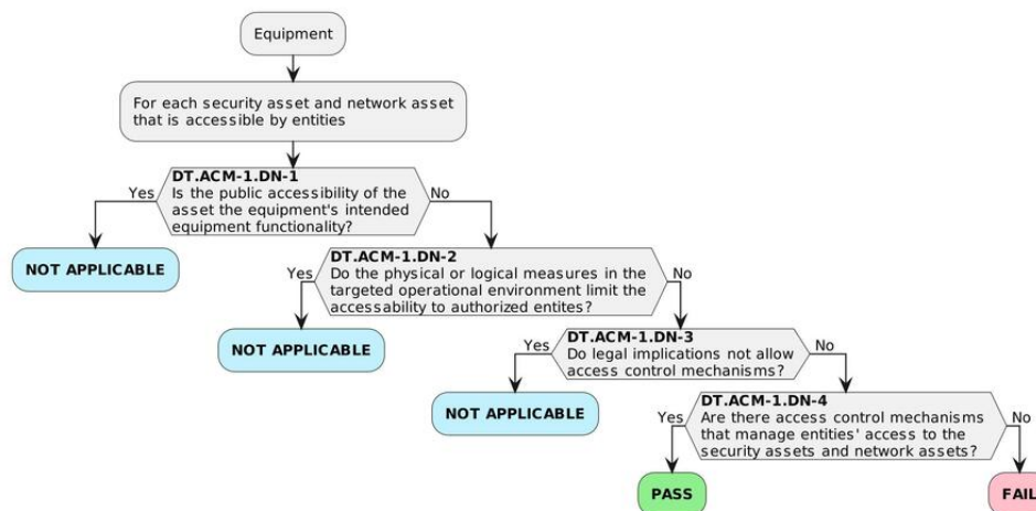
Figure 1 — Decision Tree for requirement ACM-1
