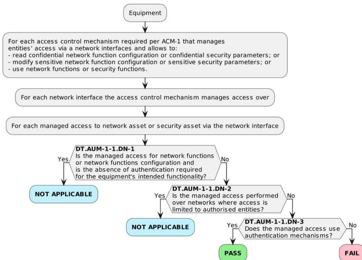
Figure 3 — Decision Tree for requirement AUM-1-1
