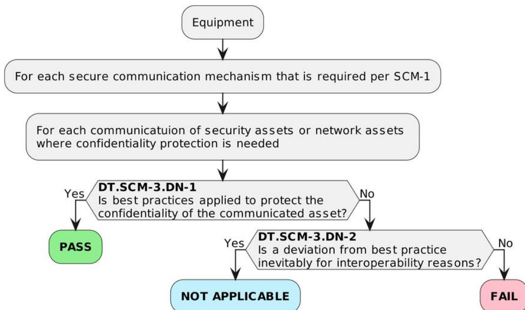
Figure 191 — Decision tree for requirement SCM-3
