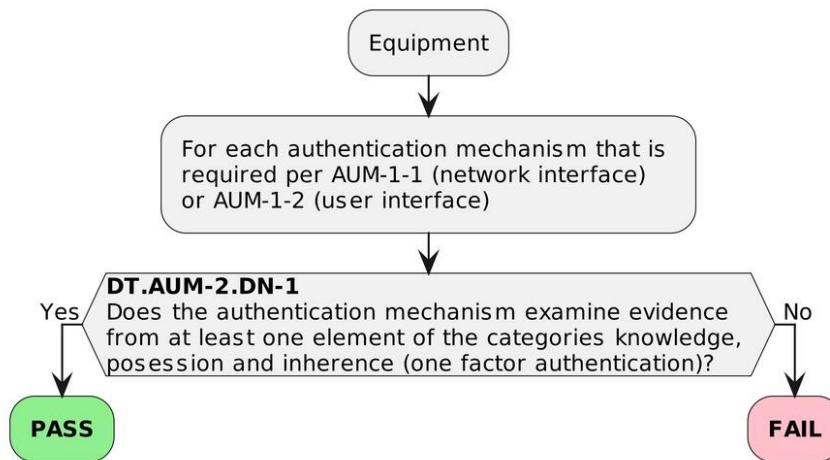
Figure 5 — Decision Tree for requirement AUM-2
