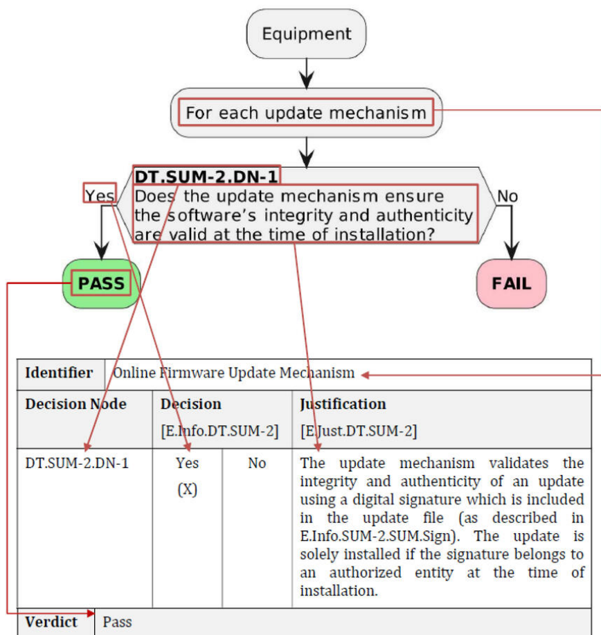
Figure A.4 — Example: Decision Tree Evidence
