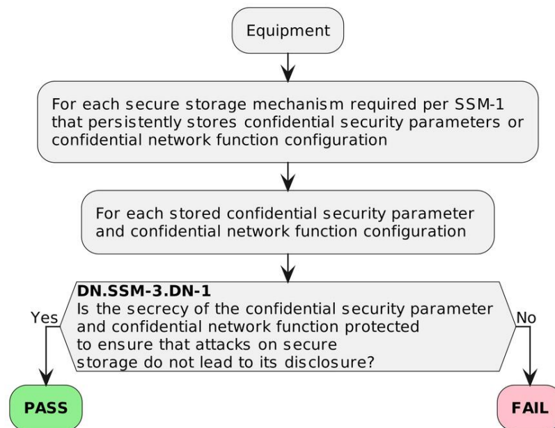
Figure 16 — Decision tree for requirement SSM-3
