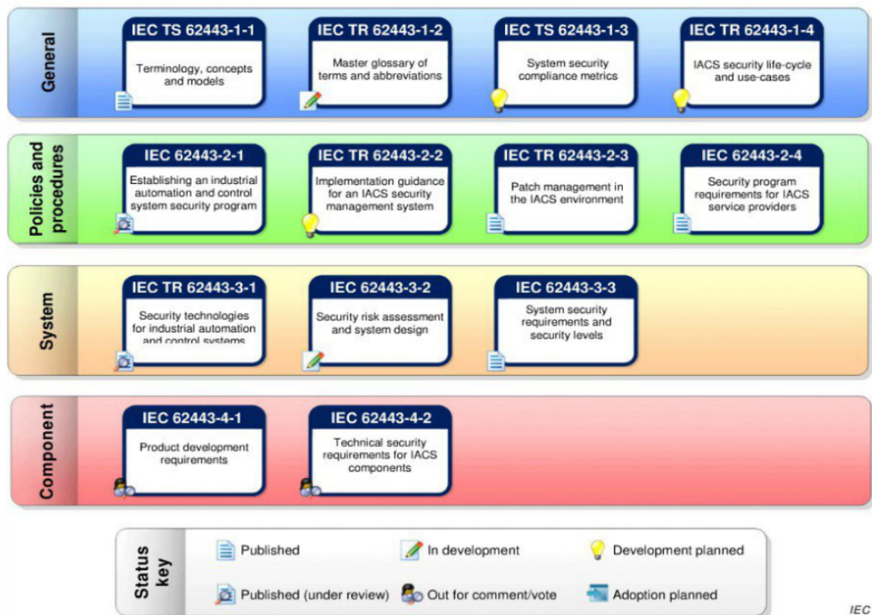
Figure 1 – Parts of the IEC 62443 series
