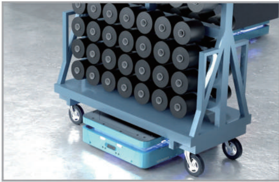
Transport the fully loaded cart with Lift AMR
