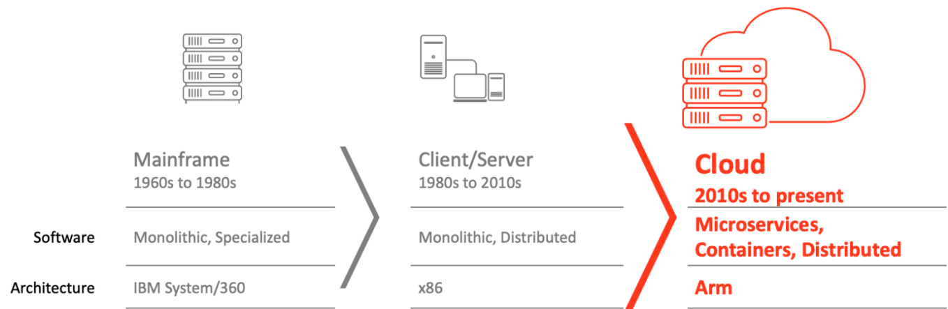
Figure 1: Compute Progression
