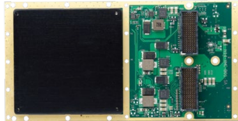
XMC-G745-R2 (conduction cooled)
