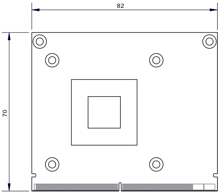
Figure 1-2: EGX-MXM-A1000/A2000 Dimensions
