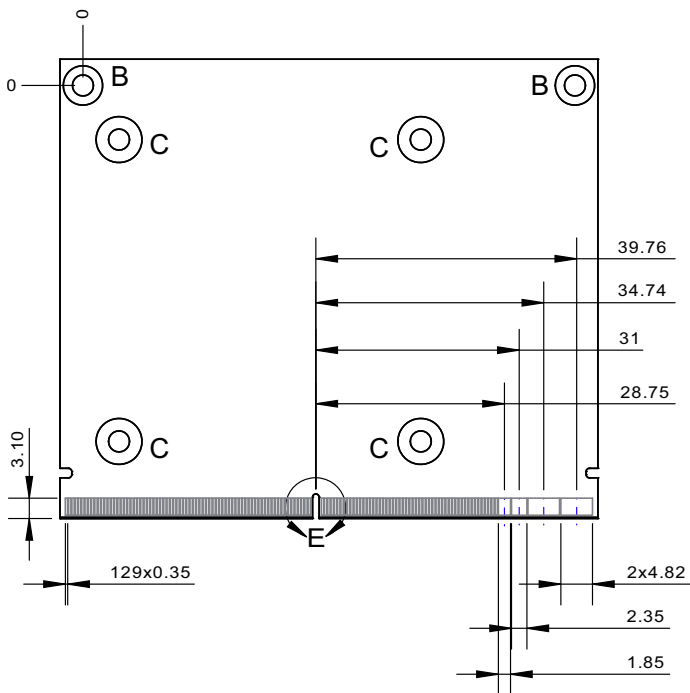
Figure 1-4: EGX-MXM-A1000/A2000 Bottom View
