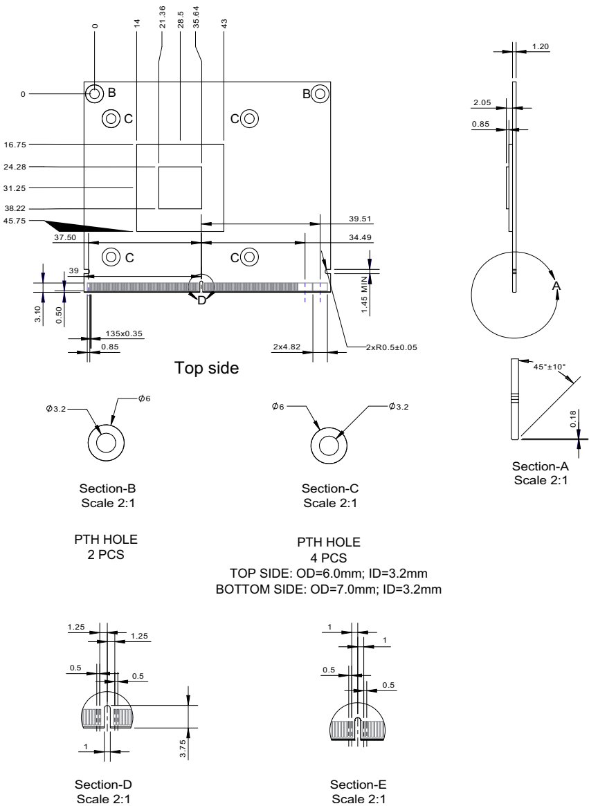
Figure 1-3: EGX-MXM-A1000/A2000 Top and Side Views
