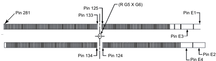
Figure 1-5: MXM Connector
