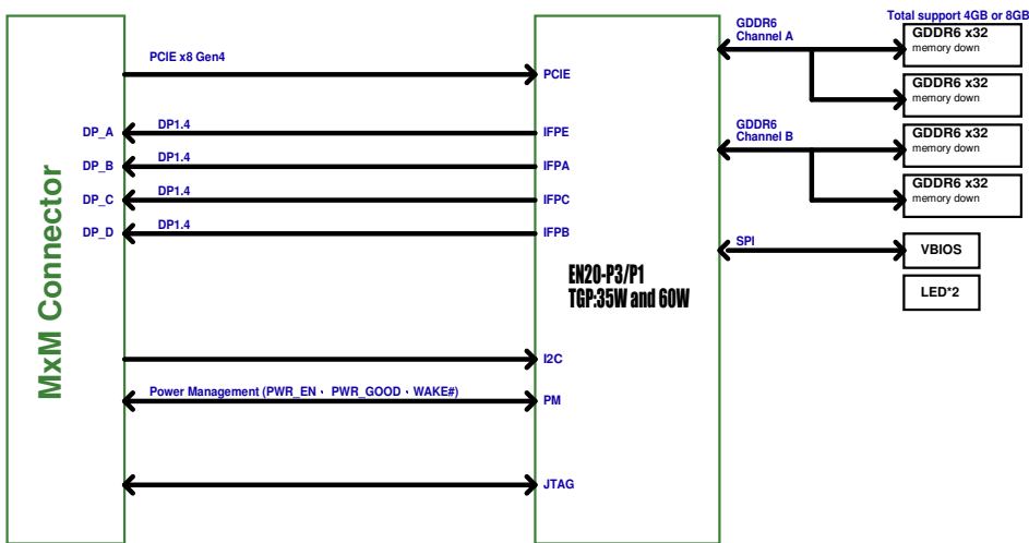
Figure 1-1: EGX-MXM-A1000/A2000 Functional Block Diagram
