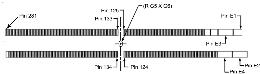
Figure 1-5: MXM Connector
