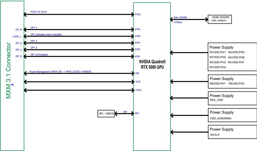
Figure 1-1: EGX-MXM-RTX5000 Functional Block Diagram
