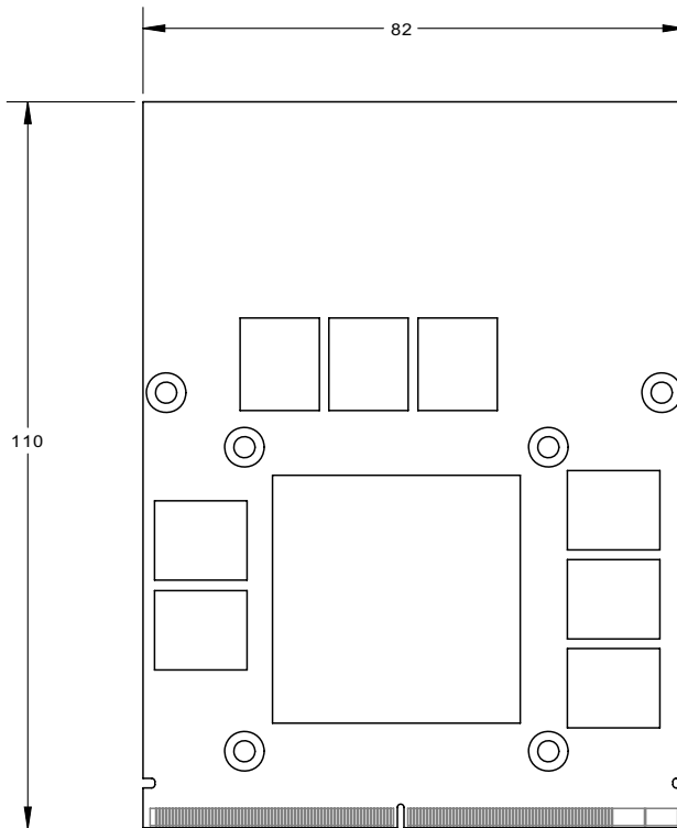
Figure 1-2: EGX-MXM-RTX5000 Dimensions
