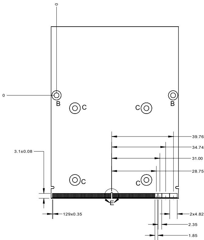
Figure 1-4: EGX-MXM-RTX5000 Layout - Bottom View
