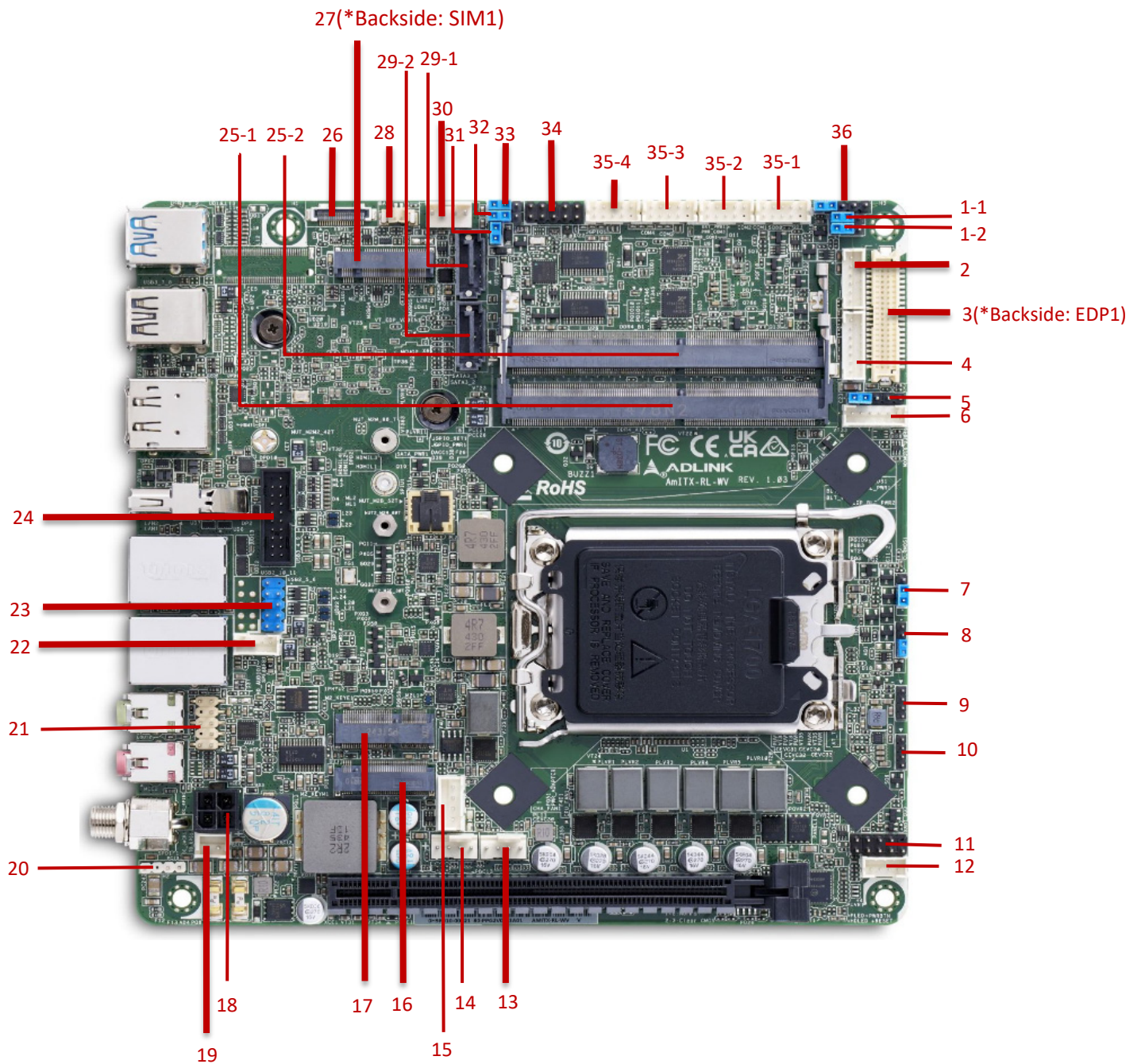
Figure 3: AmITX-RL-WV component-side connectors
