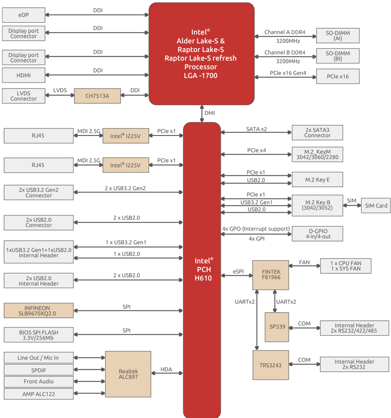
Figure 1: AmITX-RL-WV functional block diagram
