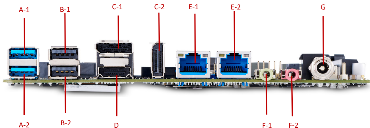
Figure 2: AmITX-RL-WV rear I/O
