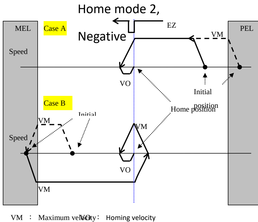
Figure 13 Home mode 2(EZ), negative direction
