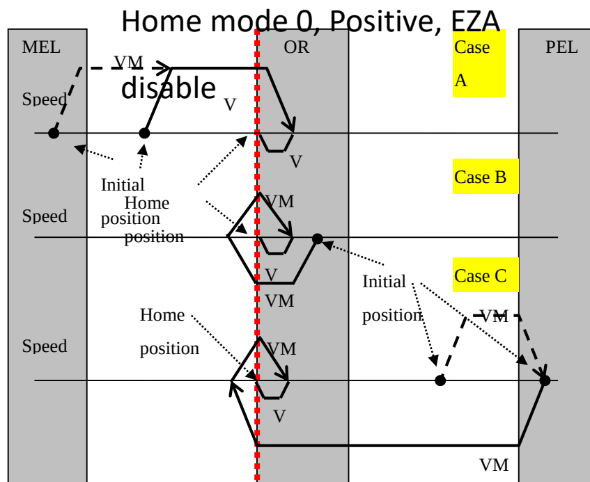
Figure 2 Home mode 0(ORG), positive direction, EZA disable
