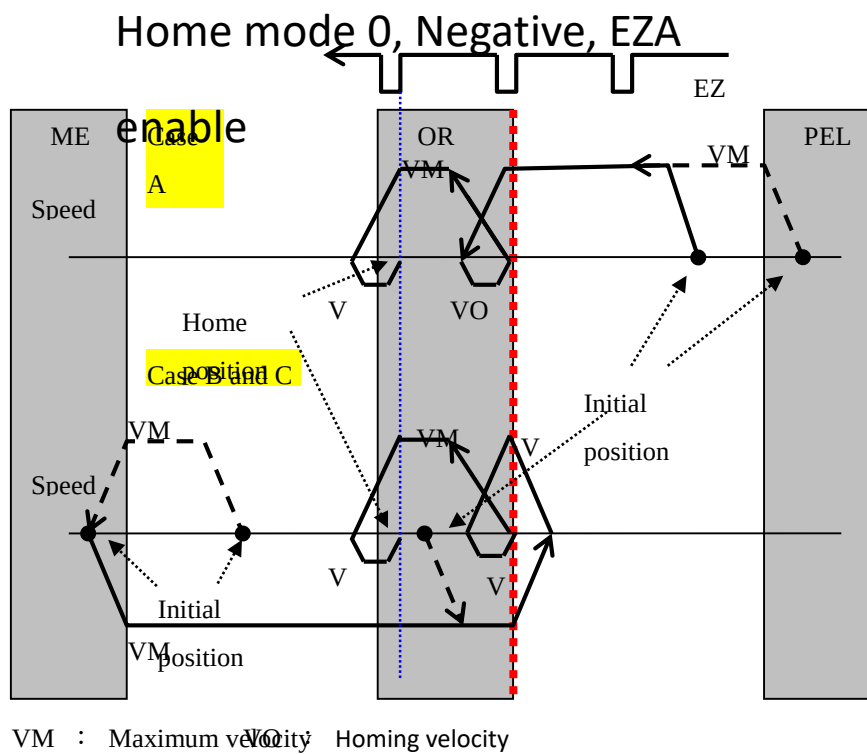
Figure 5 Home mode 0(ORG), negative direction, EZA enable, EZ_DIR disable
