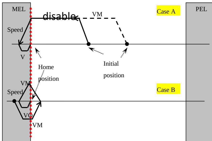
Figure 9 Home mode 1(EL), negative direction, EZA disable
