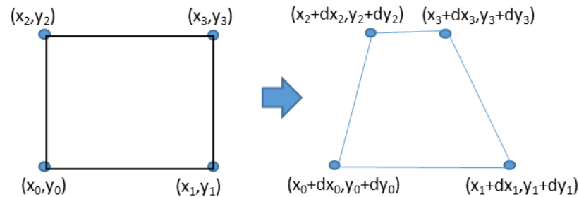
Figure 2 Example of 2-D compensation table configuration
