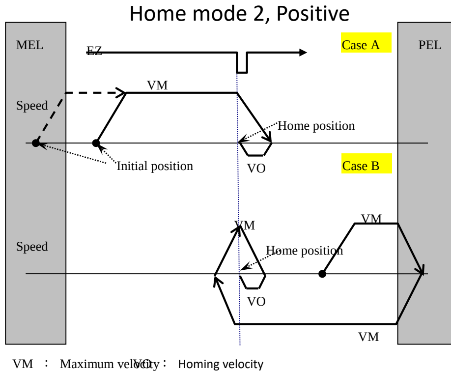
Figure 12 Home mode 2(EZ), position direction
