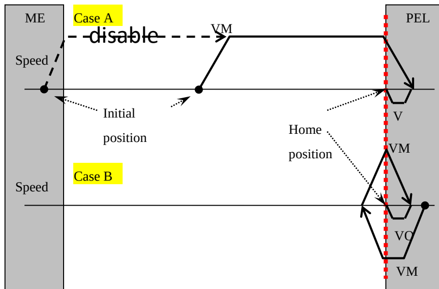
Figure 8 Home mode 1(EL), positive direction, EZA disable
