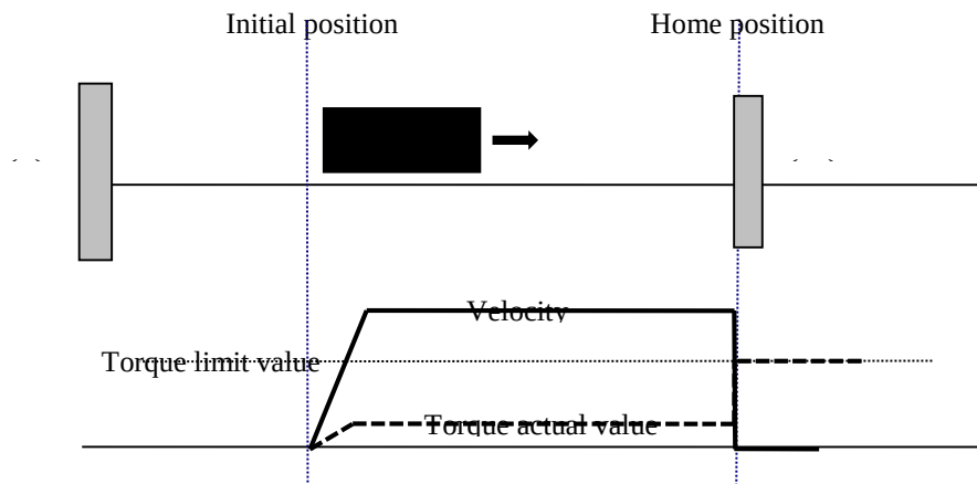
Figure 14 Home mode 3(torque), positive direction
