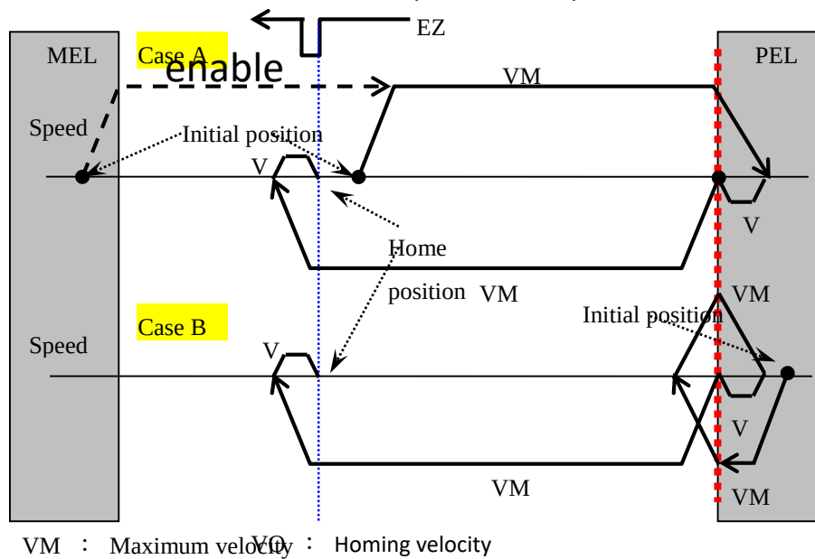
Figure 10 Home mode 1(EL), positive direction, EZA enable
