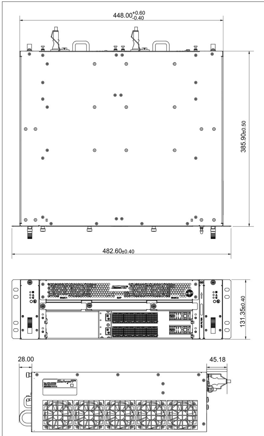
Figure 18: AC-System
