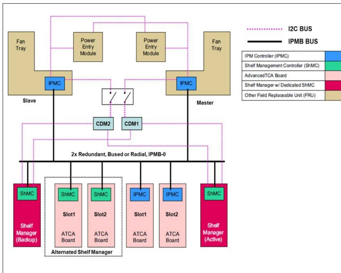
Figure 14: Shelf Management
