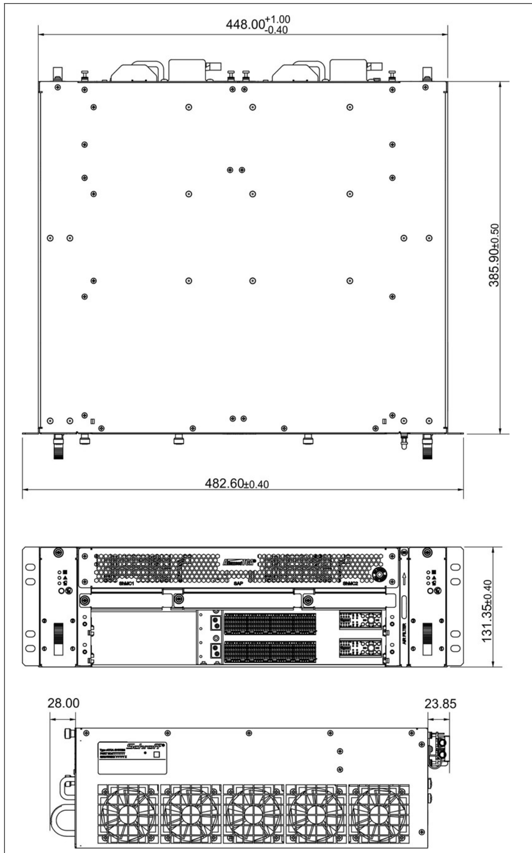
Figure 17: DC-System
