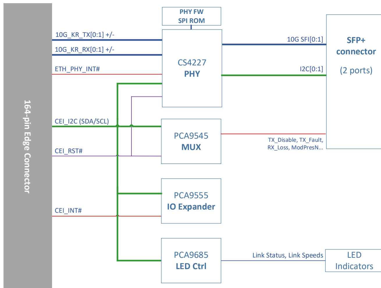
Figure 1 – CEI-2x10G SFP+ function diagram
