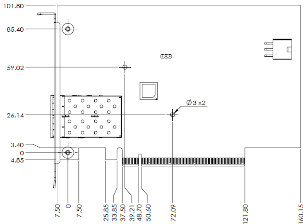
Figure 4 – CEI-2x10G SFP+ mechanical dimensions
