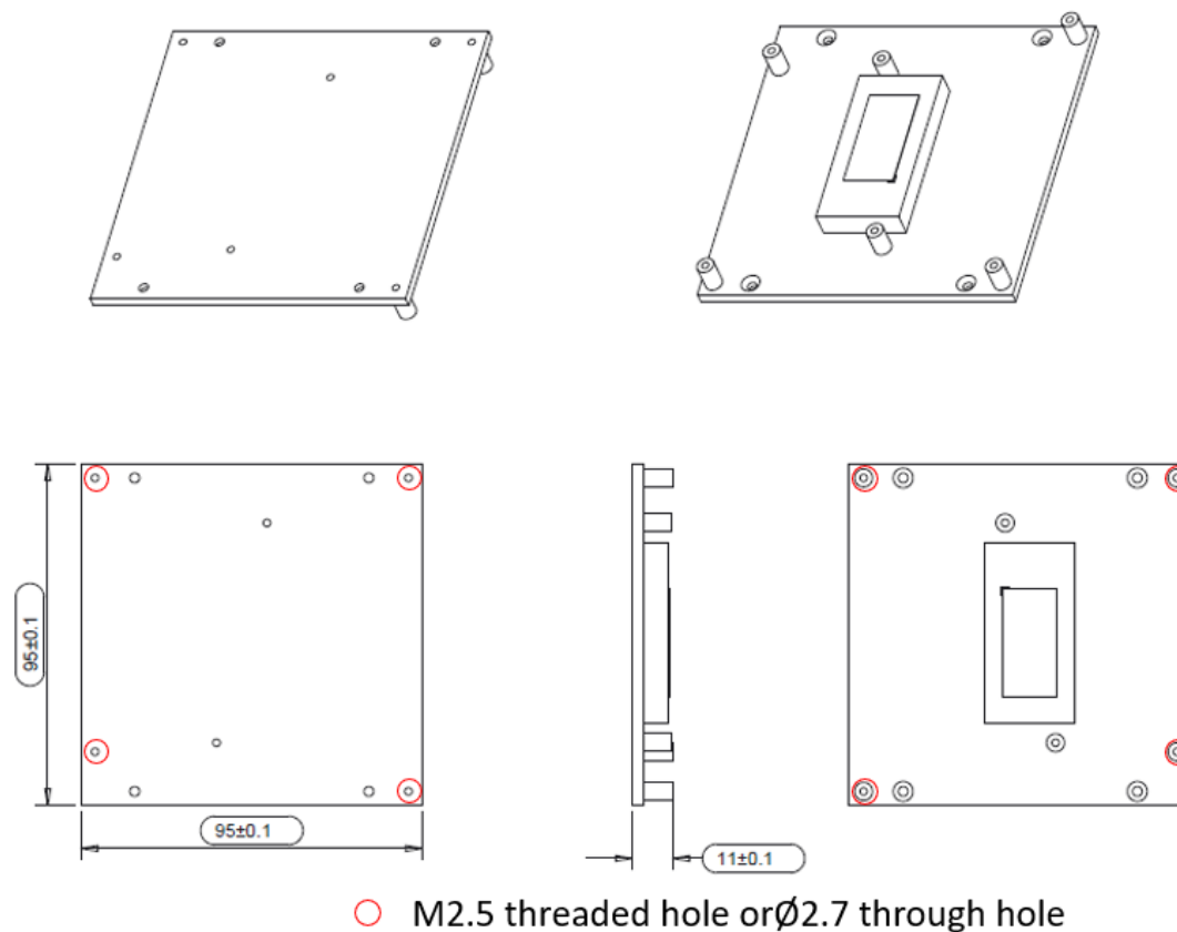
Figure 6 – Heatspreader: HTS
