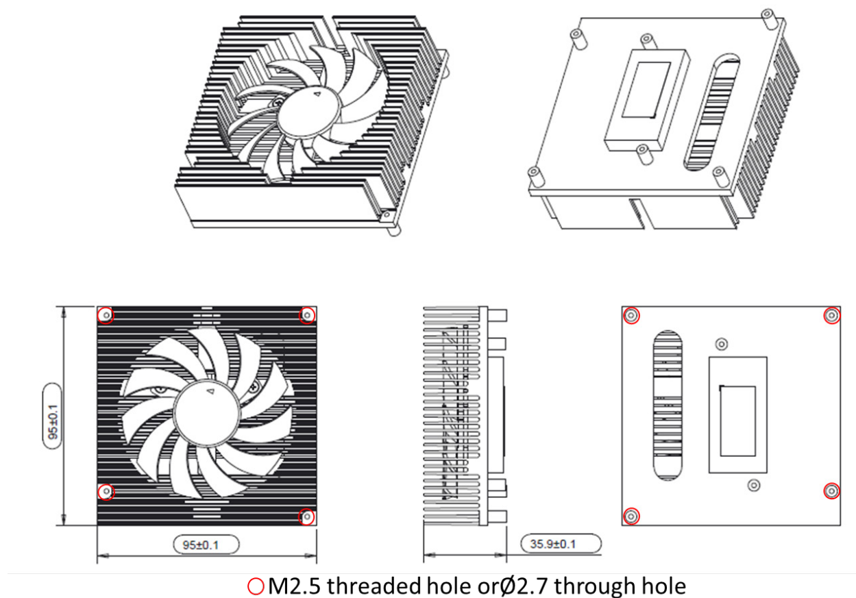
Figure 9 – Heatsink with fan: THSF
