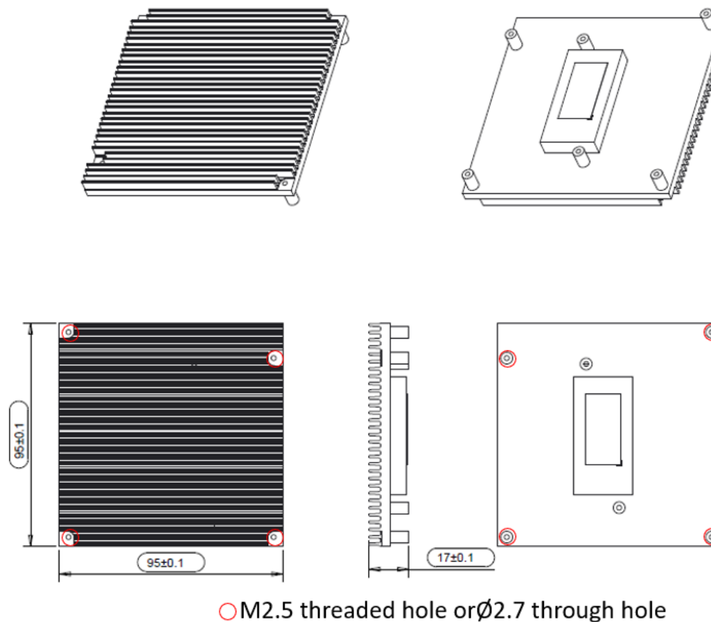
Figure 7 – Heatsink: THS
