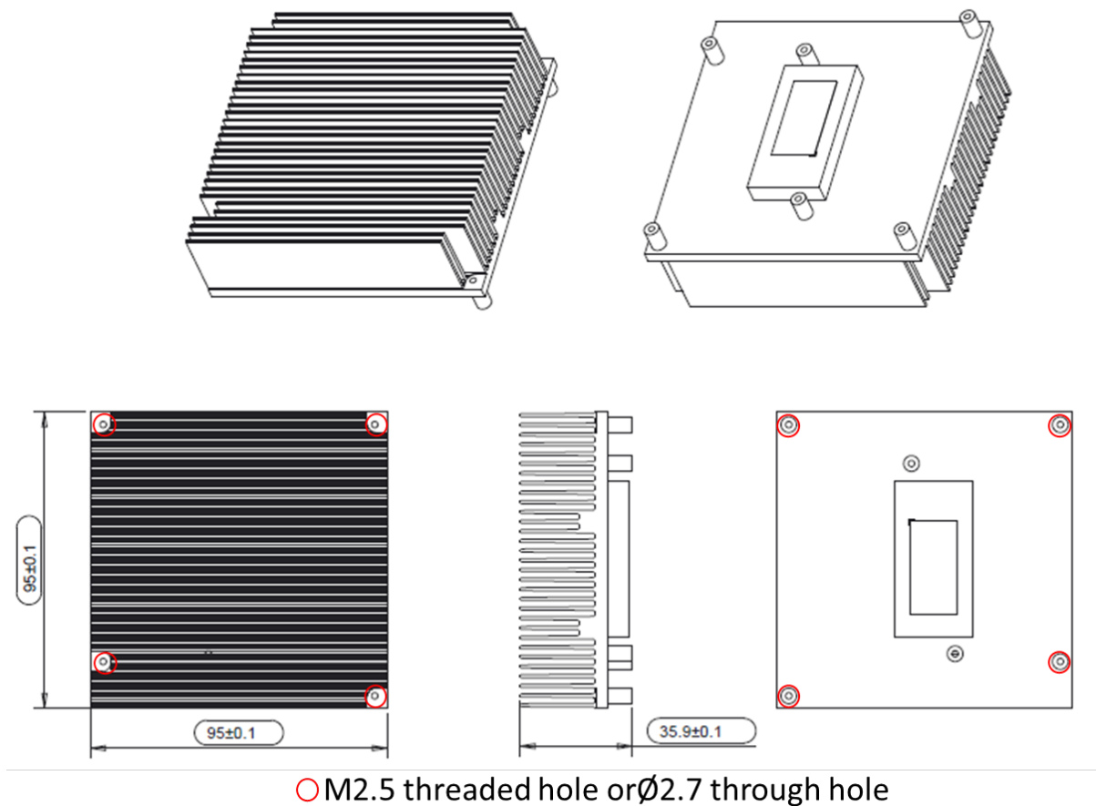
Figure 8 – Heatsink high profile: THSH
