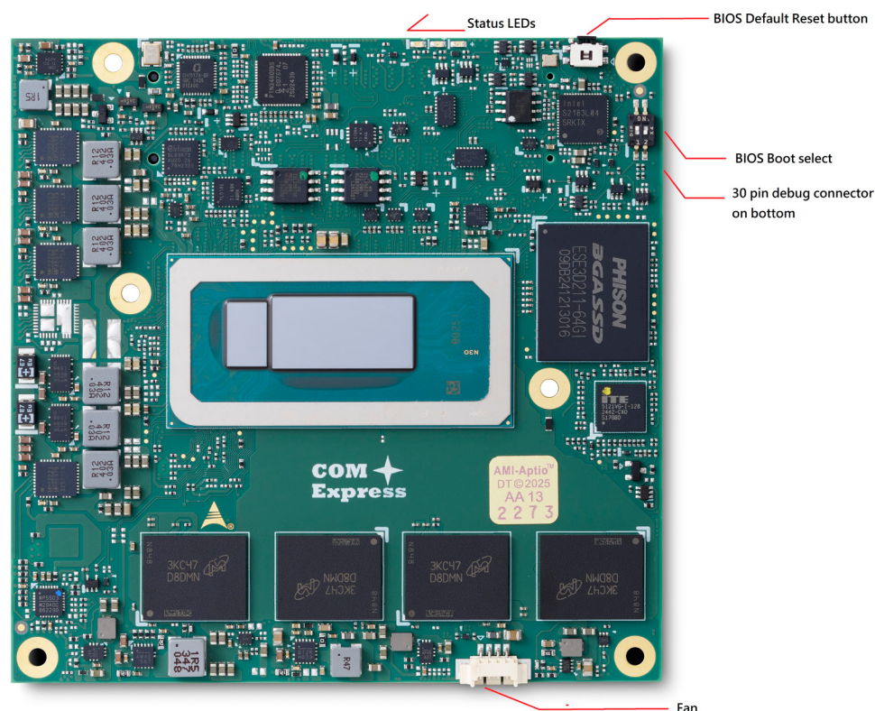
Figure 3 – Module feature locations (top side)
