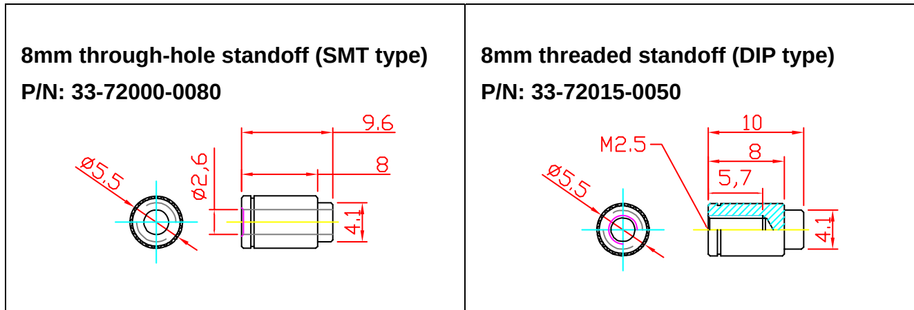
Figure 7: COM Express Standoff Types
