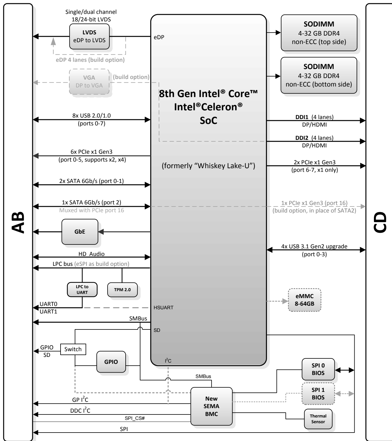
Figure 1: cExpress-WL Functional Block Diagram
