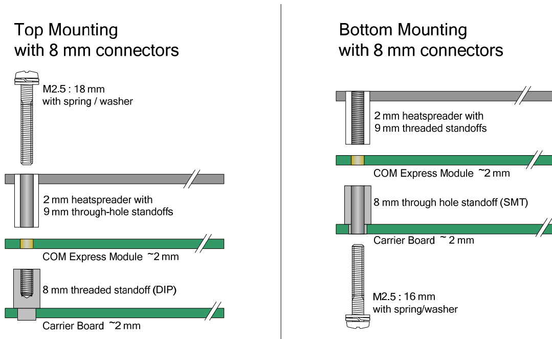
Figure 6: COM Express Mounting Methods
