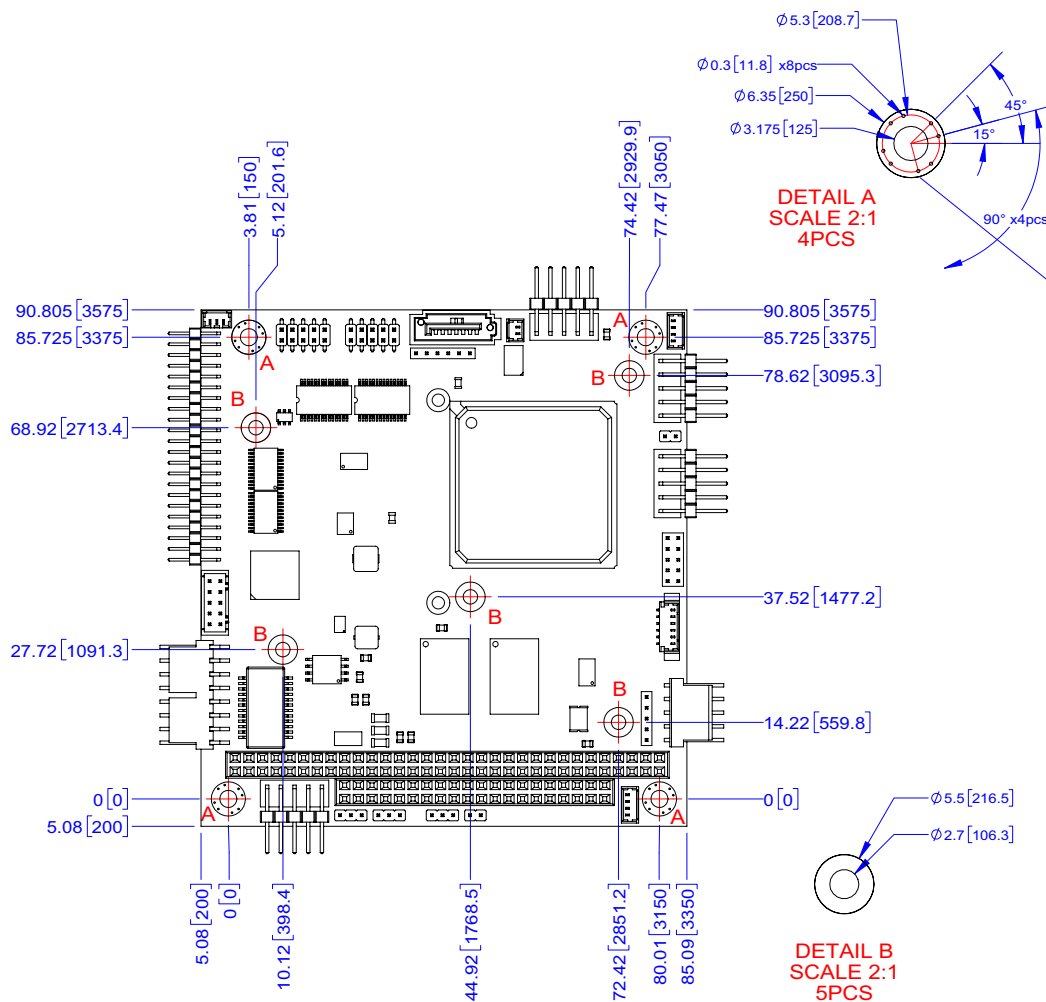
Figure 1-2: Mechanical Overview (Top Side)
