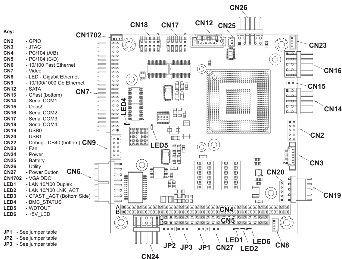
Figure 2-3: Header, Connector, and Socket Locations (Top Side)
