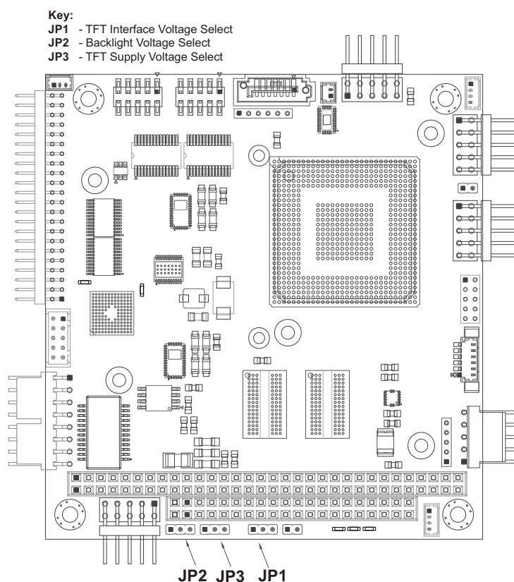
Figure 2-5: Jumper Header Locations (Top Side)
