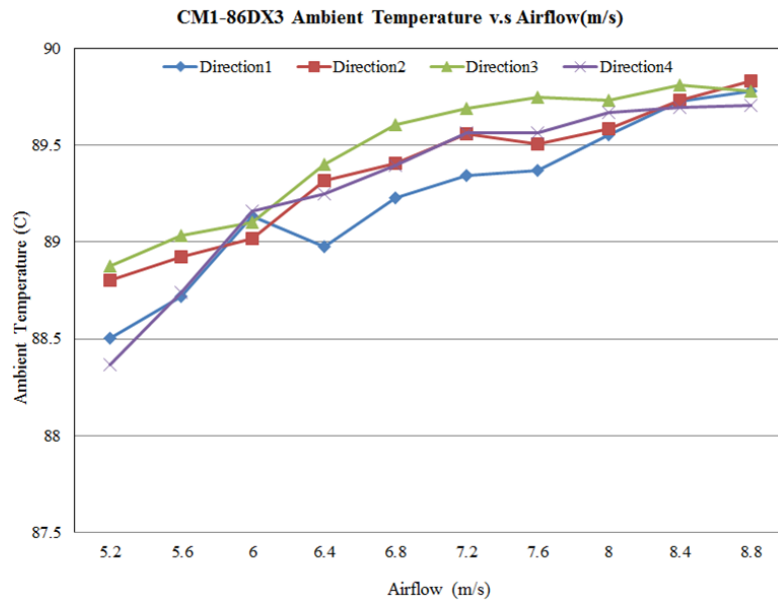
Figure 1-4: Temperature vs Airflow Chart
