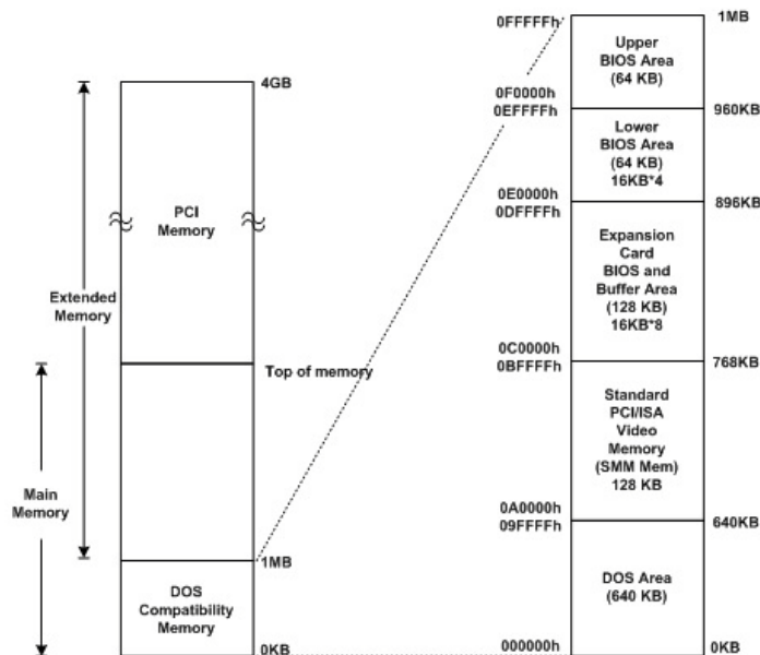
Figure B-2: Memory Address Map
