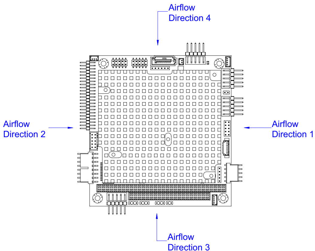
Figure 1-5: Airflow Directions with CM1-86DX3-TM Heatsink
