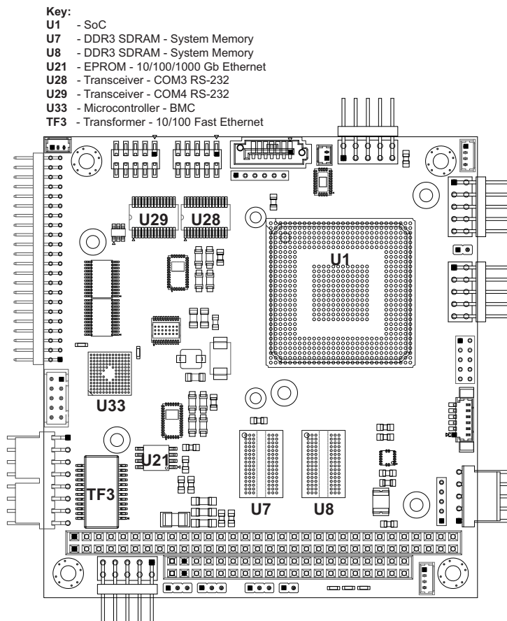
Figure 2-1: Component Locations (Top Side)
