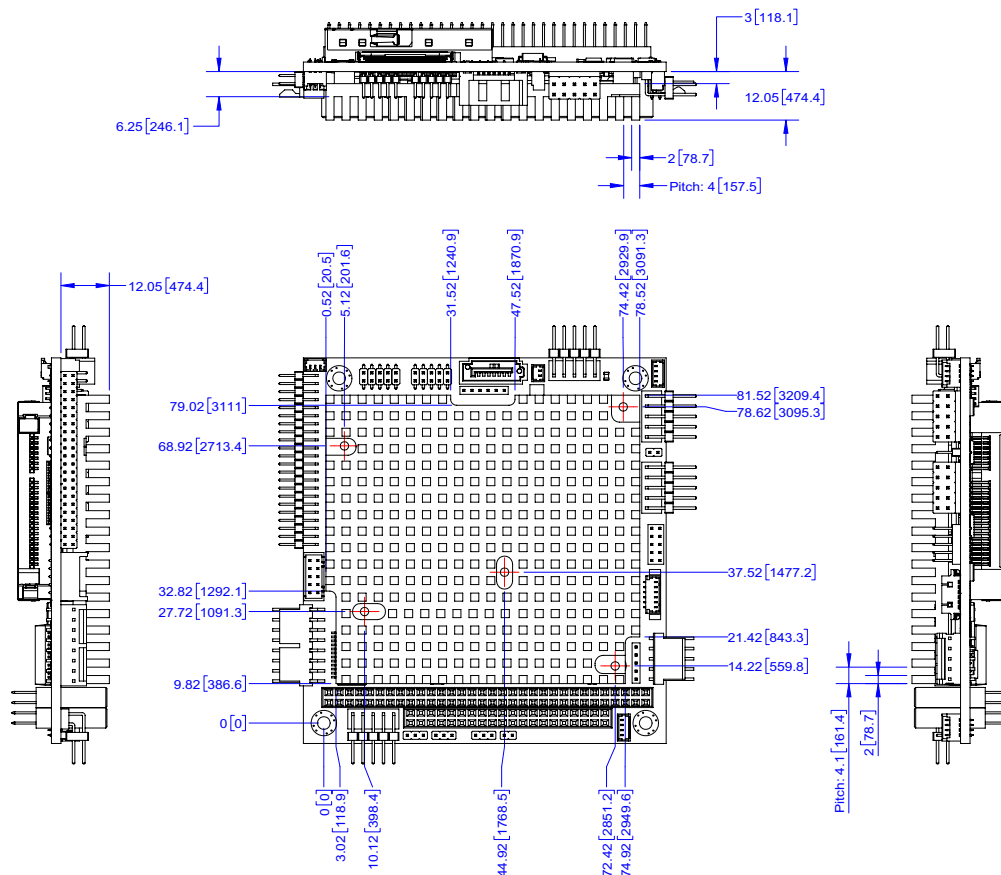
Figure 1-3: Heatsink mounting dimensions (top side)
