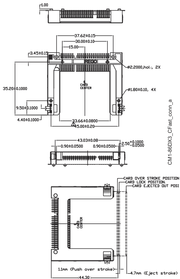
Figure 2-6: CFast Slot
