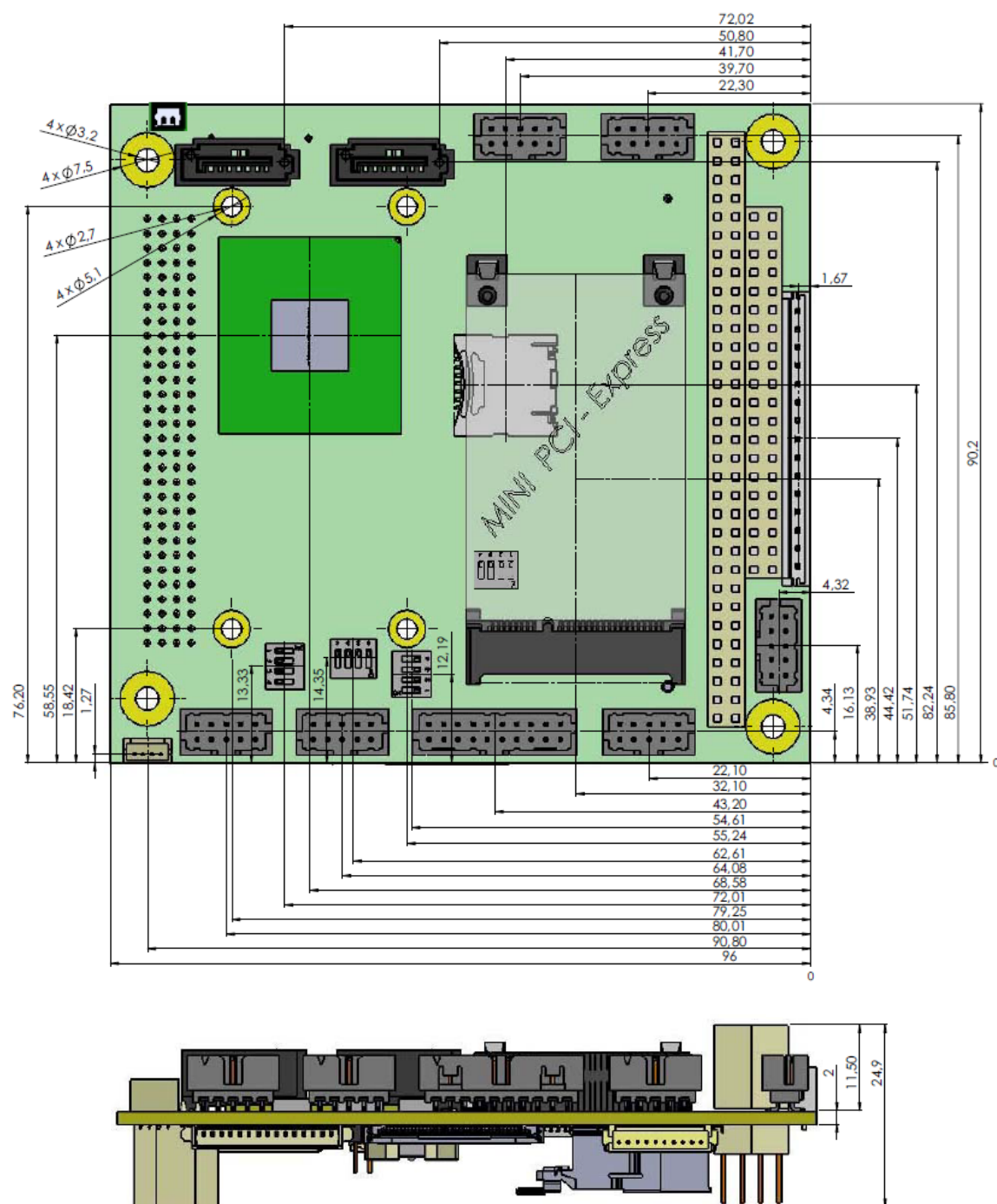
Figure 2-3: Mechanical Dimensions
