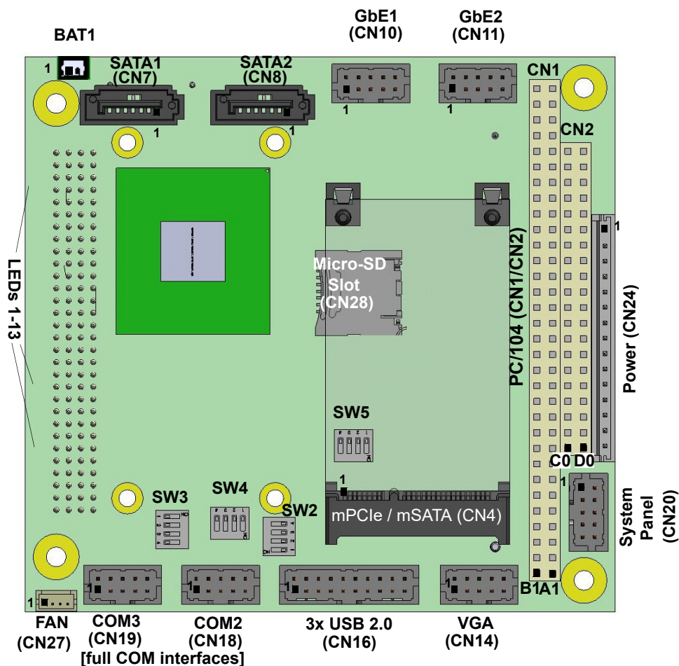
Figure 2-1: Header and Connector Locations (Top Side)
