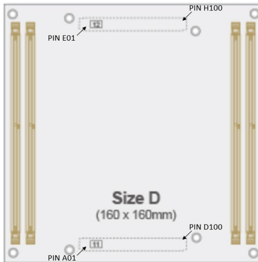
Figure 2 - Module rear side row and pin numbering
