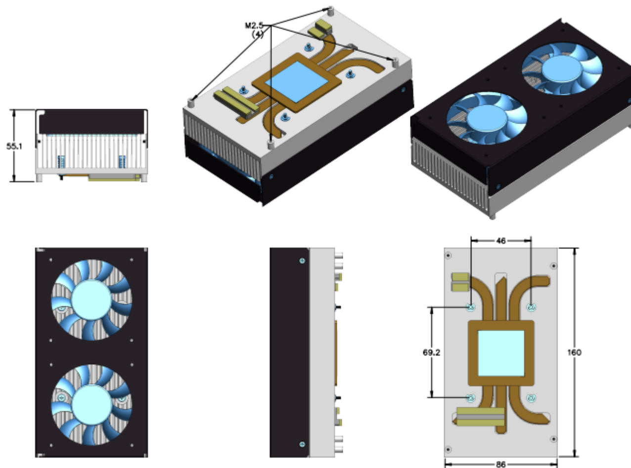
Figure 8 – Heatsink with Fan: THSF
