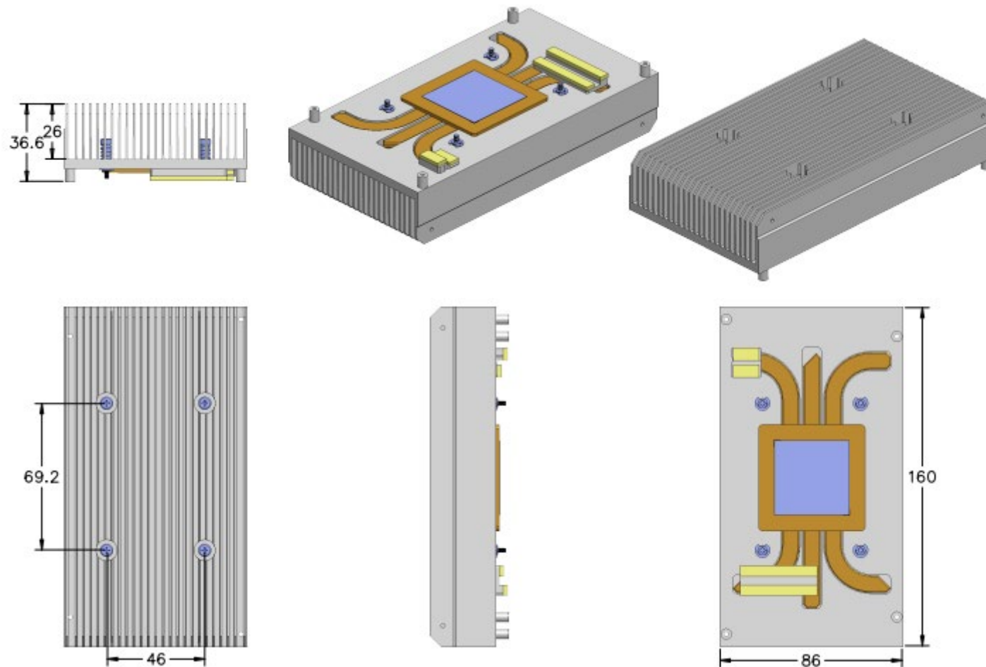
Figure 7 – Heatsink: THS-BL
