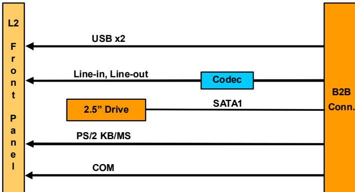
Figure 2-2: cPCI-3620D Daughter Board Functional Block Diagram
