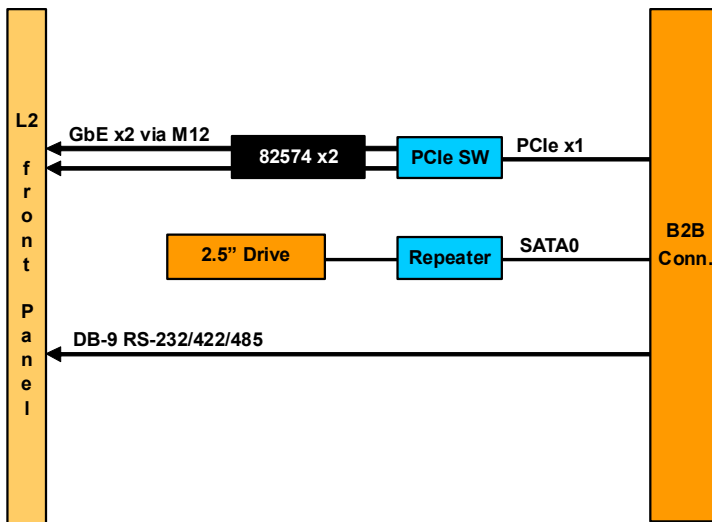
Figure 2-3: cPCI-3620T Daughter Board Functional Block Diagram
