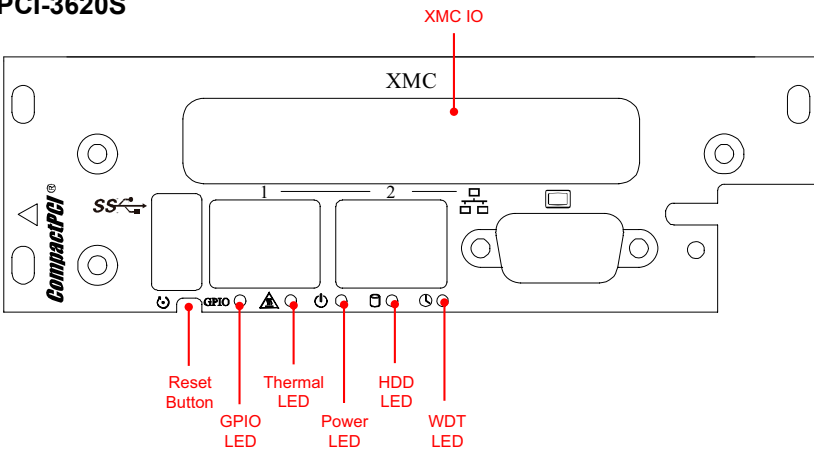
Figure 4-7: cPCI-3620T, cPCI-3620S Faceplate Layout
