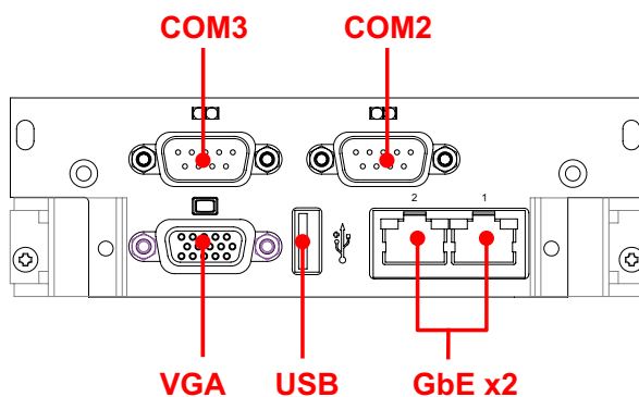
Figure 4-9: cPCI-R3610(T) RTM Faceplate
