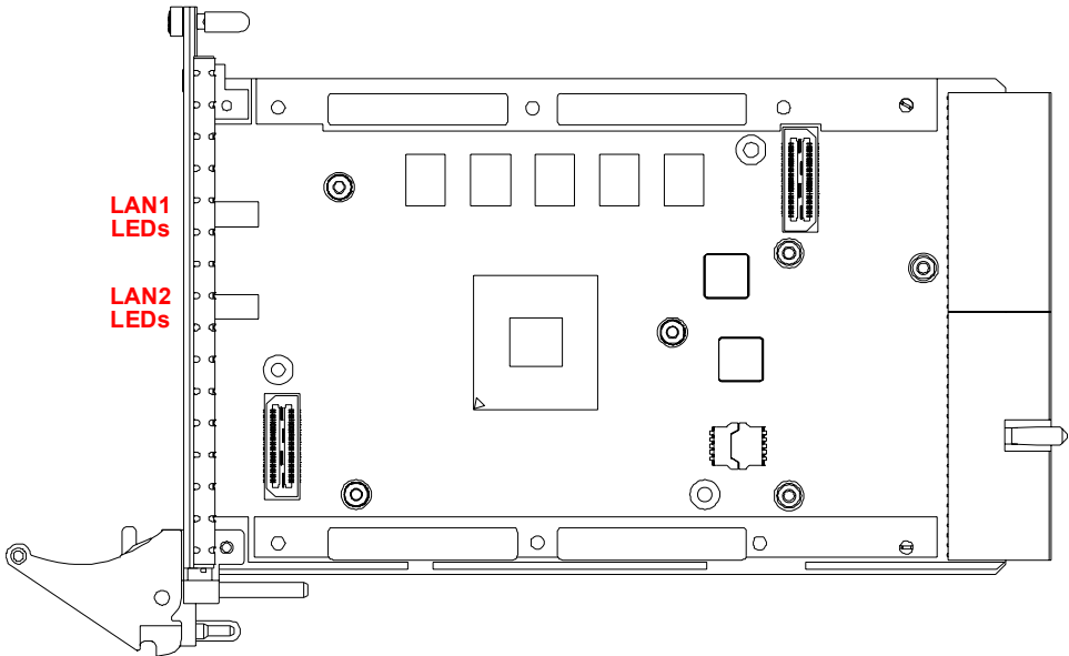
Figure 4-5: cPCI-3620N Blade Assembly Layout
