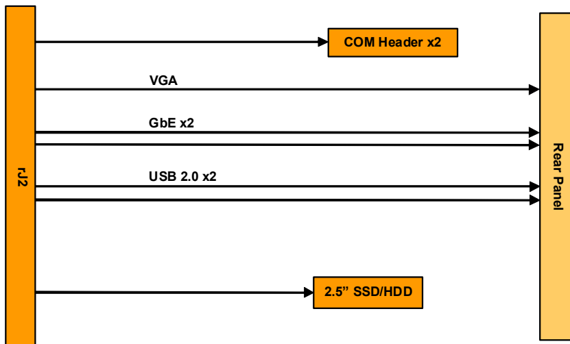
Figure 2-4: cPCI-R3610 RTM Functional Block Diagram
