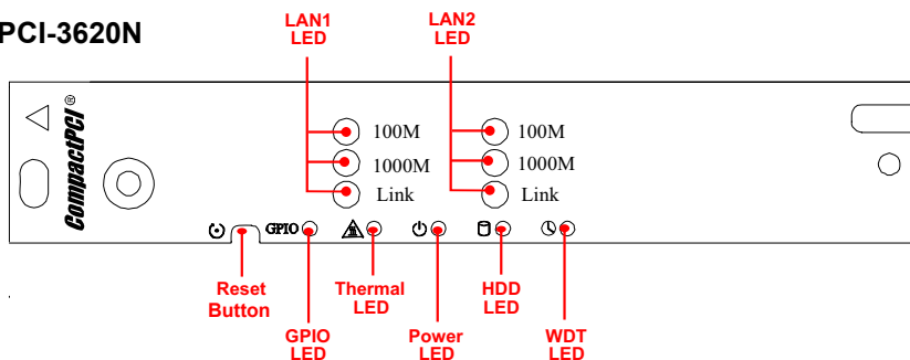
Figure 4-6: cPCI-3620, cPCI-3620D, cPCI-3620N Faceplate Layout
