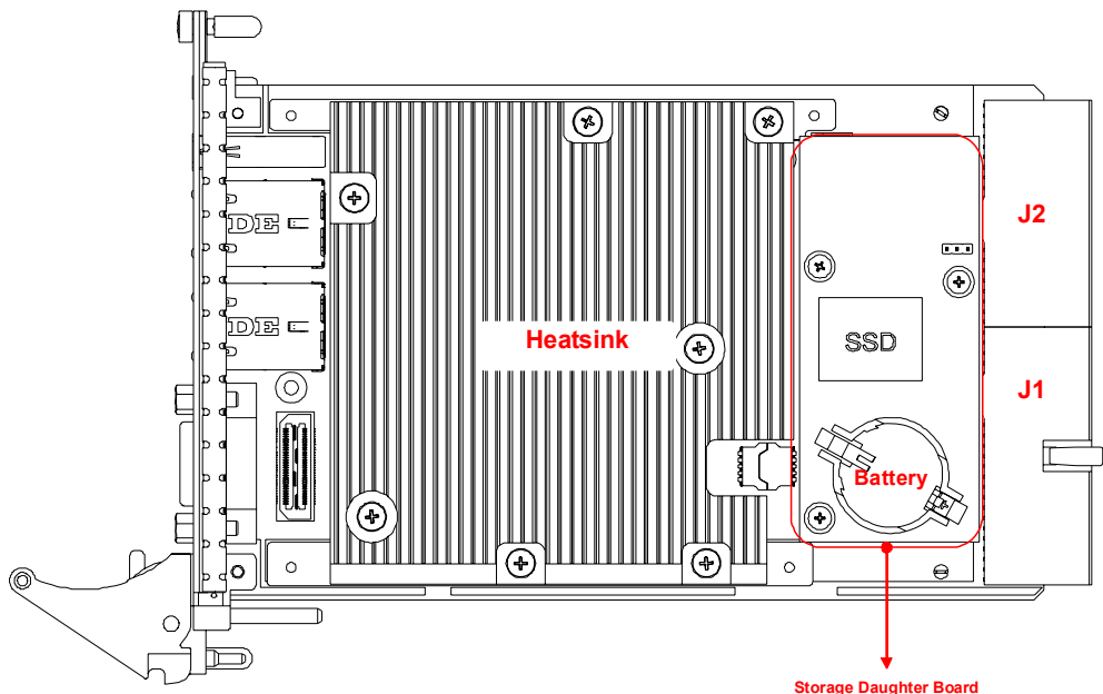
Figure 4-2: cPCI-3620 Blade Assembly Layout
