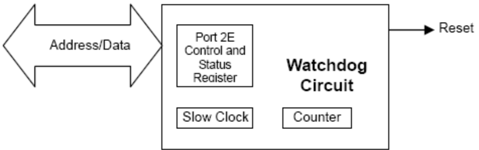
Figure 7-1: cPCI-3915 Watch Dog Timer Architecture
