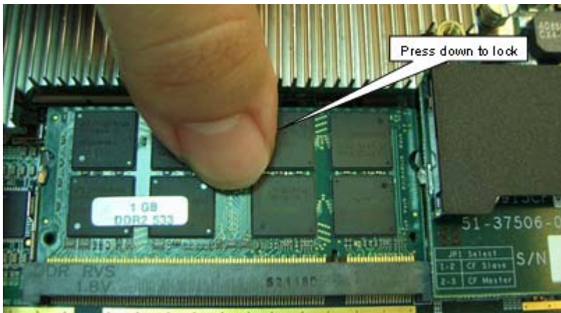
Figure 5-3: Memory Installation
