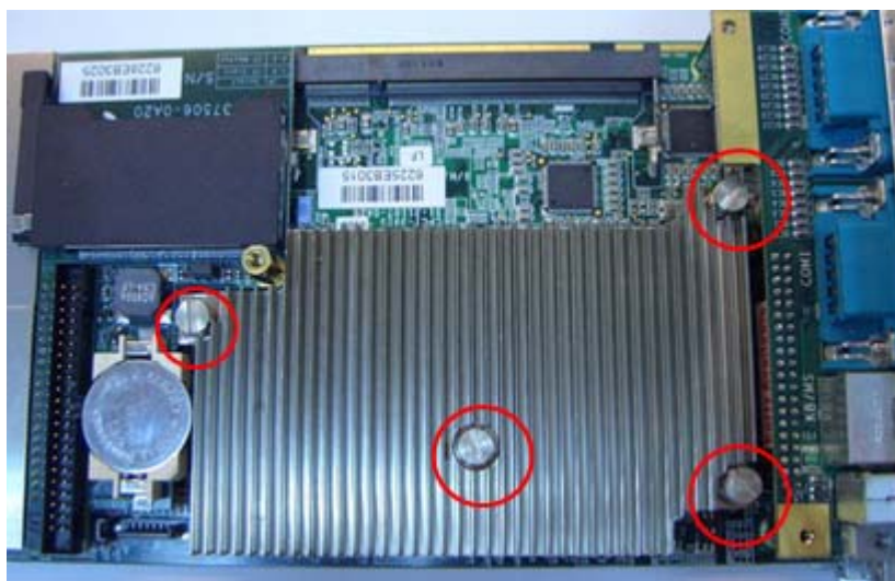
Figure 5-2: Heat Sink Installation
