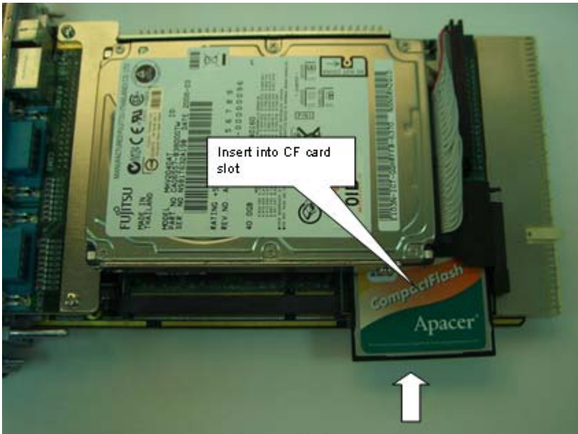
Figure 5-5: Compact Flash Card Installation
