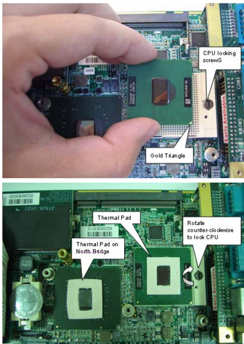
Figure 5-1: CPU Installation
