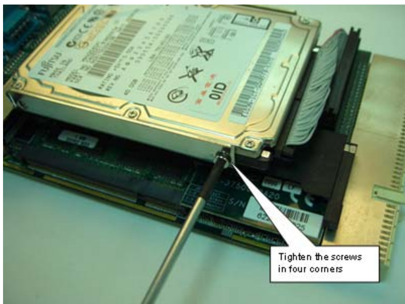
Figure 5-4: 2.5" Hard Disk Installation
