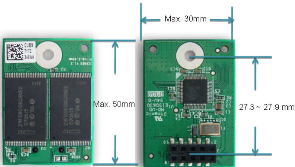
Figure 3-2: USB Flash Disk Mechanical Layout
