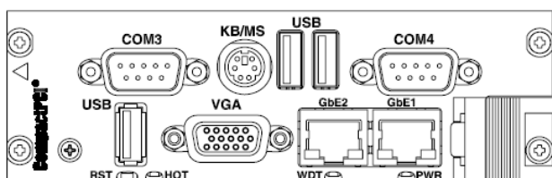
Figure 2-6: cPCI-3920B Assembly and Front Panel
