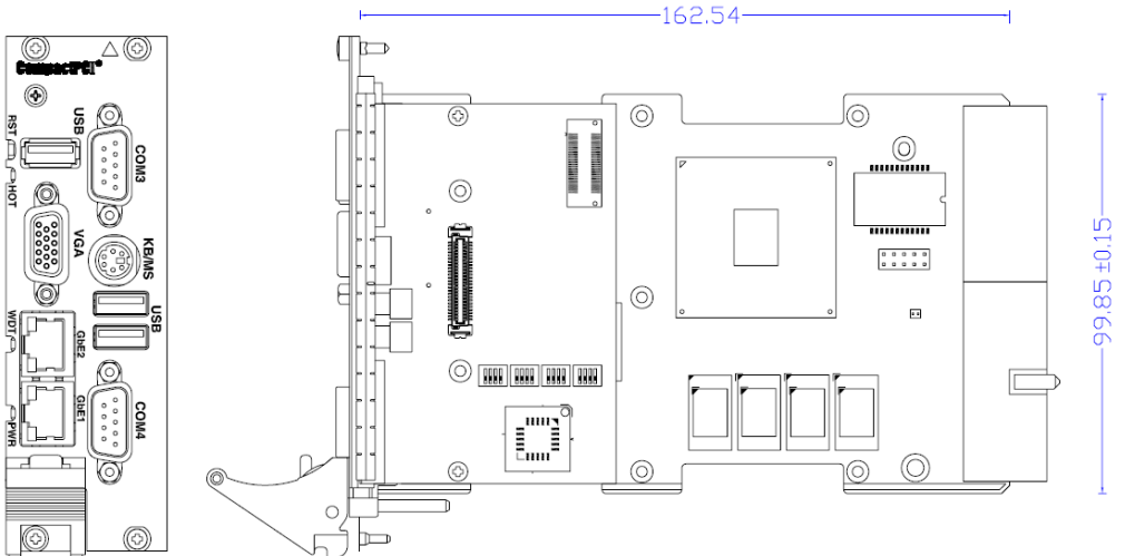
Figure 2-1: cPCI-3920 Mechanical Dimensions
