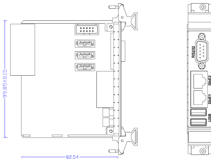
Figure 2-2: cPCI-R3920 Mechanical Dimensions
