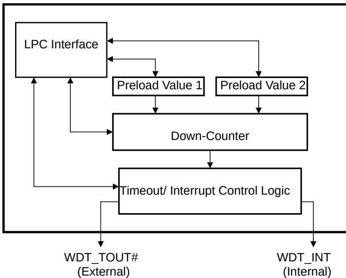
Figure 6-1: cPCI-3920 Watchdog Timer Architecture
