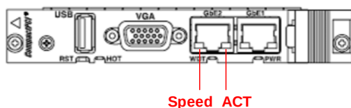
Figure 2-4: cPCI-3920A Assembly and Front Panel
