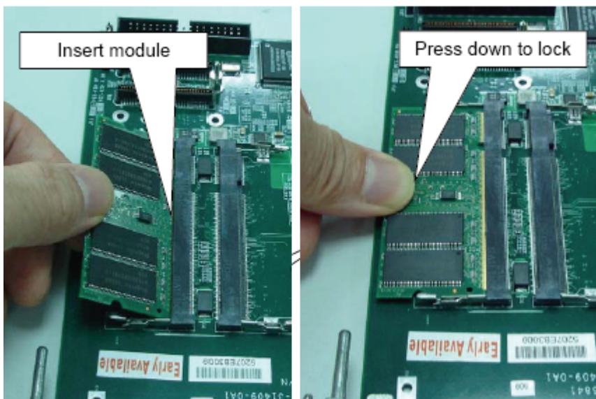
Figure 3-3: Memory Installation
