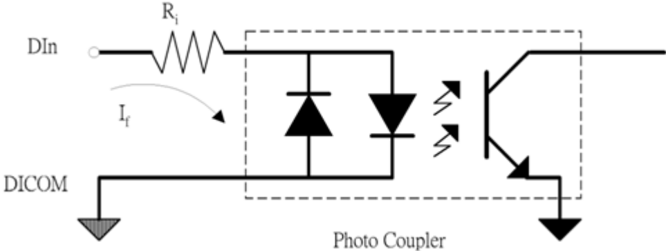
Figure 4-1: Photo Coupler
