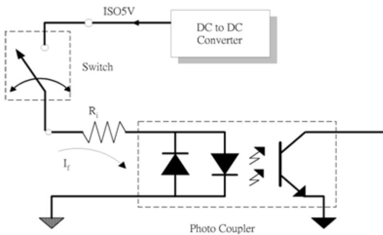
Figure 4-2: Dry Contact
