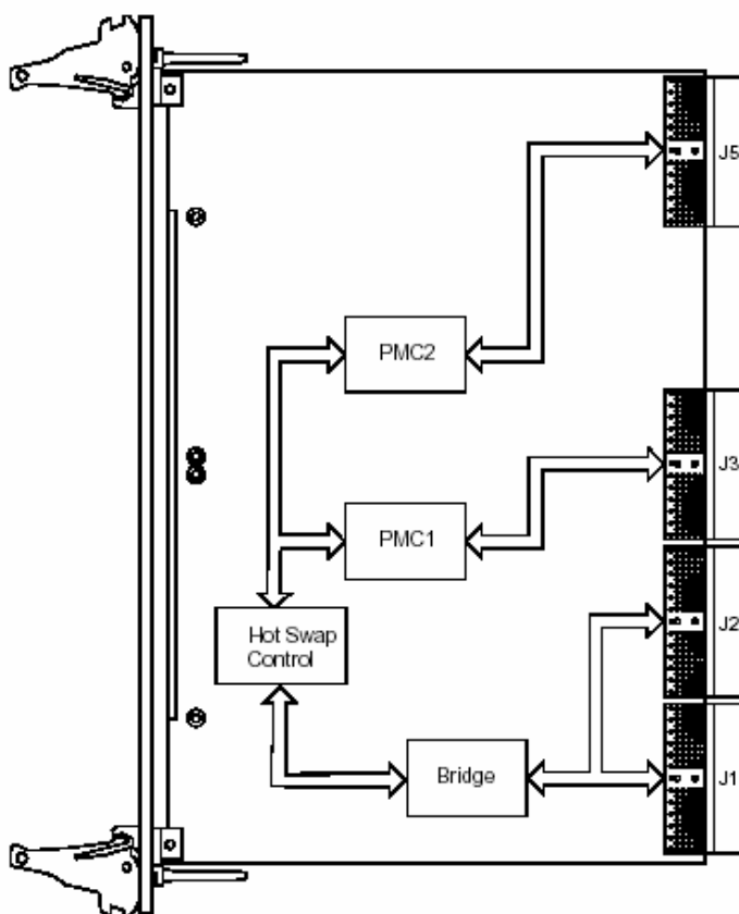
Figure 2.2 cPCI-6802 Functional Layout
