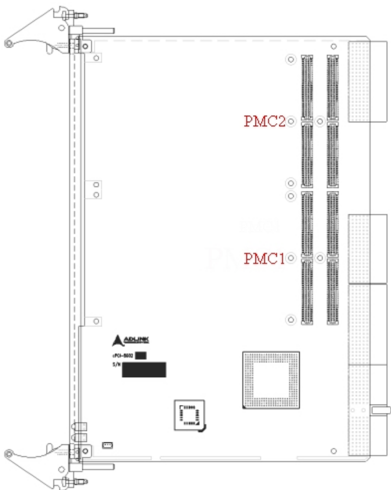
Figure 2.1 cPCI-6802 Layout
