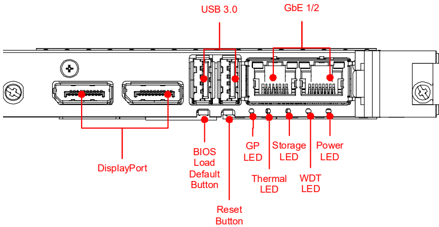
Figure 3-3: cPCI-A3525 Faceplate Layout
