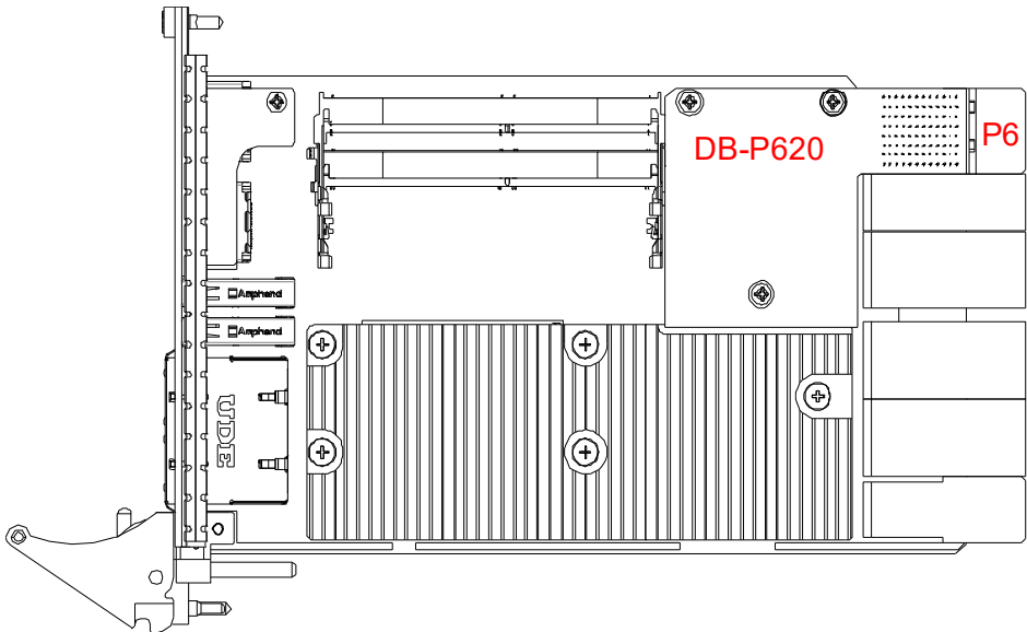
Figure 3-2: cPCI-A3525 Blade Assembly Layout
