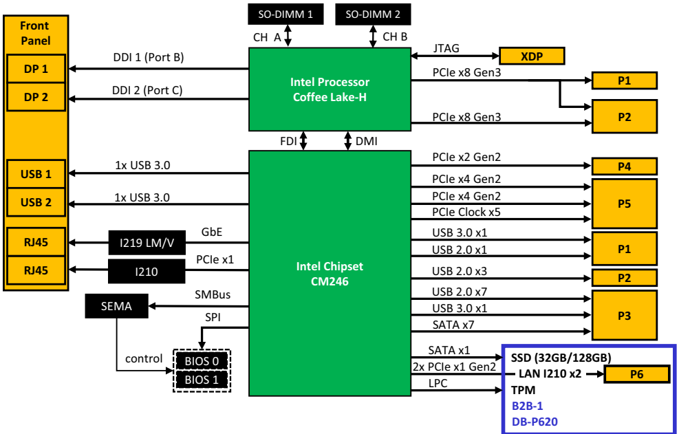
Figure 2-1: cPCI-A3525 Processor Blade Functional Block Diagram
