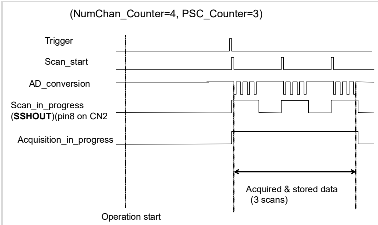
Figure 4-8: Post-trigger
