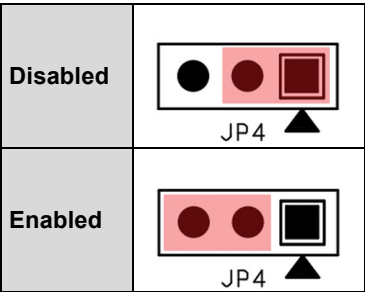
Figure 2-4: DIO Initial Status (JP4)
