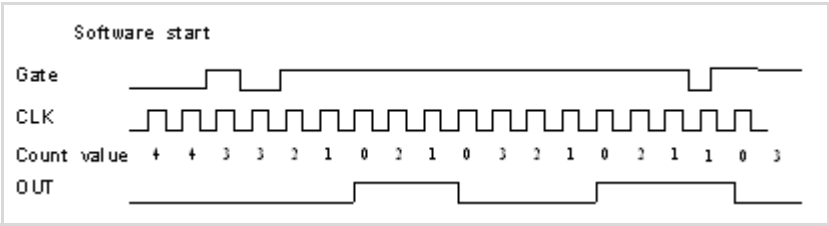
Figure 4-28: Mode 8 Operation
