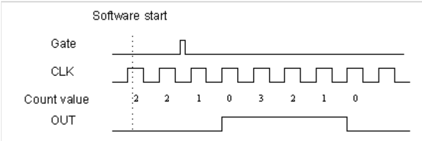
Figure 4-25: Mode 5 Operation
