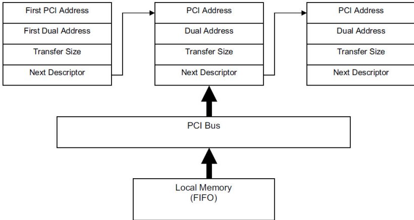
Figure 4-11: Linked List of PCI Address DMA Descriptors
