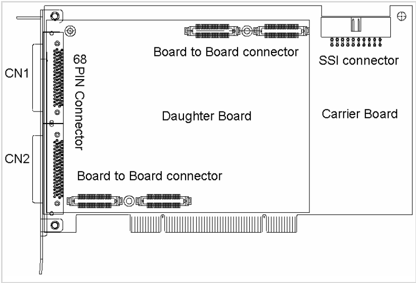
Figure 2-1: PCB Layout of DAQ/DAQe-2213/2214
