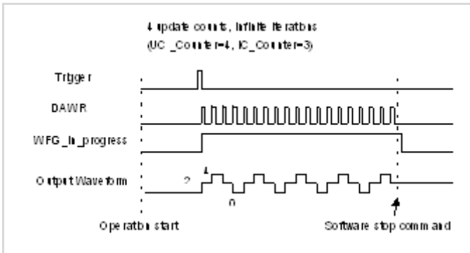
Figure 4-18: Stop Mode I
