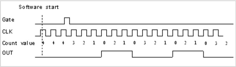
Figure 4-27: Mode 7 Operation
