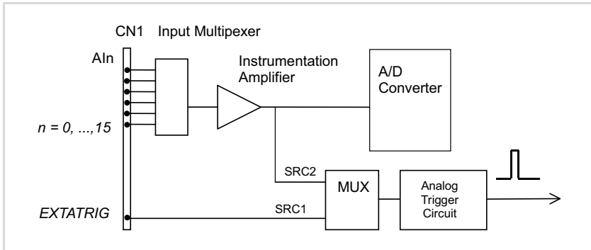
Figure 4-29: Analog Trigger Block Diagram
