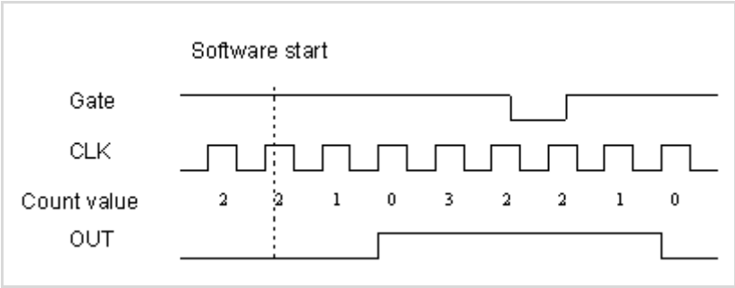
Figure 4-24: Mode 4 Operation
