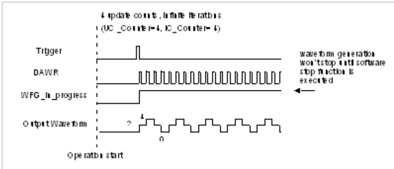
Figure 4-17: Infinite Iterative Waveform Generation with Post-trigger (DLY2_Counter = 0)
