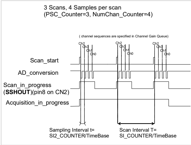
Figure 4-1: Scan Timing
