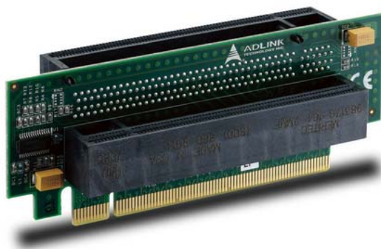
PClex16-to-two-x8 Adapter Card (Model: P16TO28, Part No.: 91-79301-0010)
