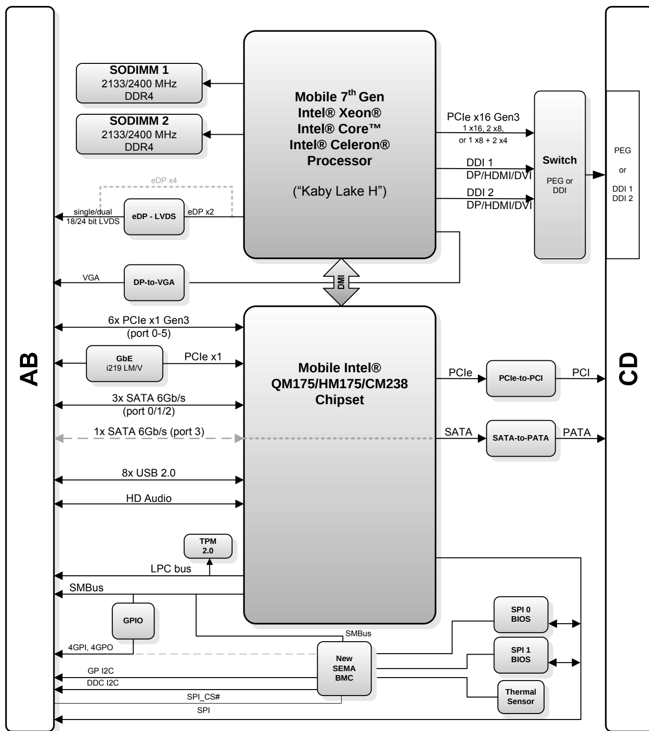
Figure 1: Express-KL2 Functional Block Diagram
