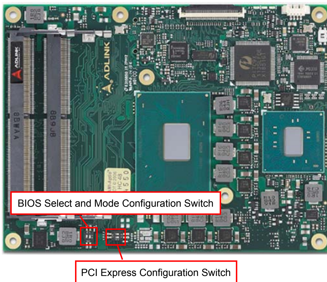
Figure 5: cExpress Switch Locations
