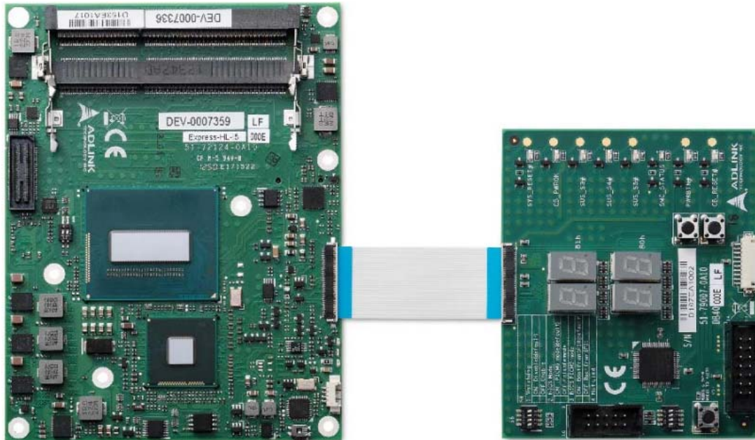
Figure 4: Express-KL2 and the DB40 Debug Module
