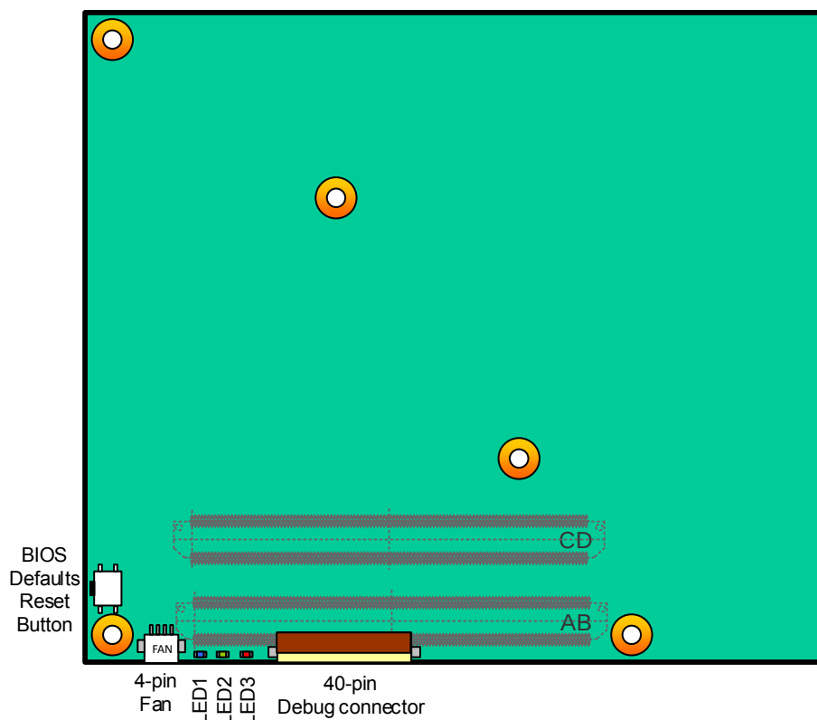
Figure 3: Express-KL2 Connector, Switch and LED Locations
