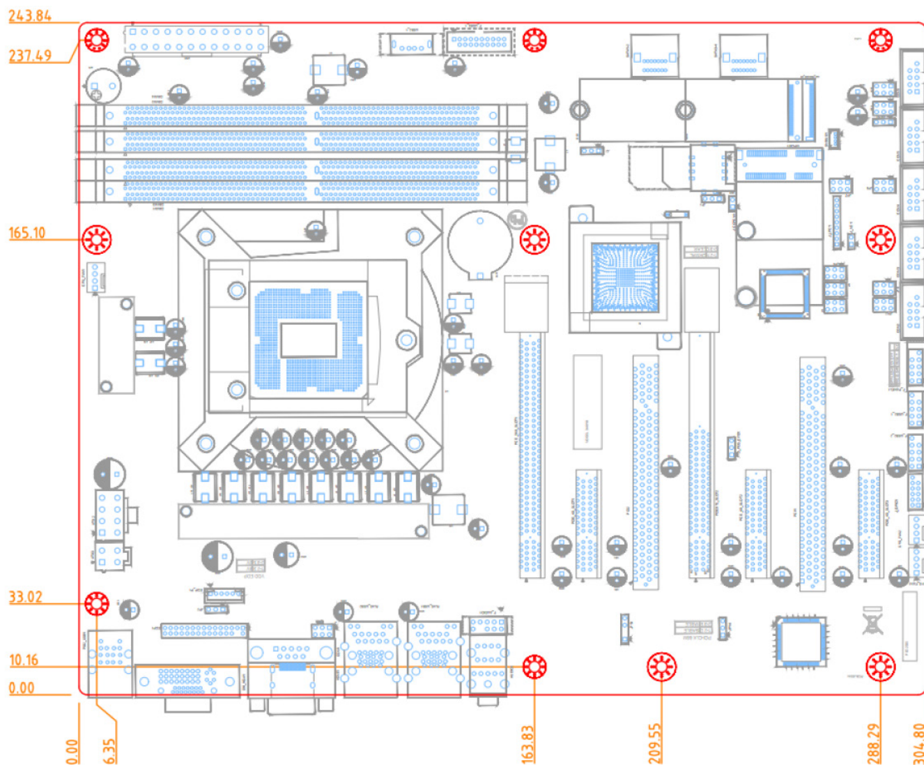
Figure 4: Mechanical Dimensions
