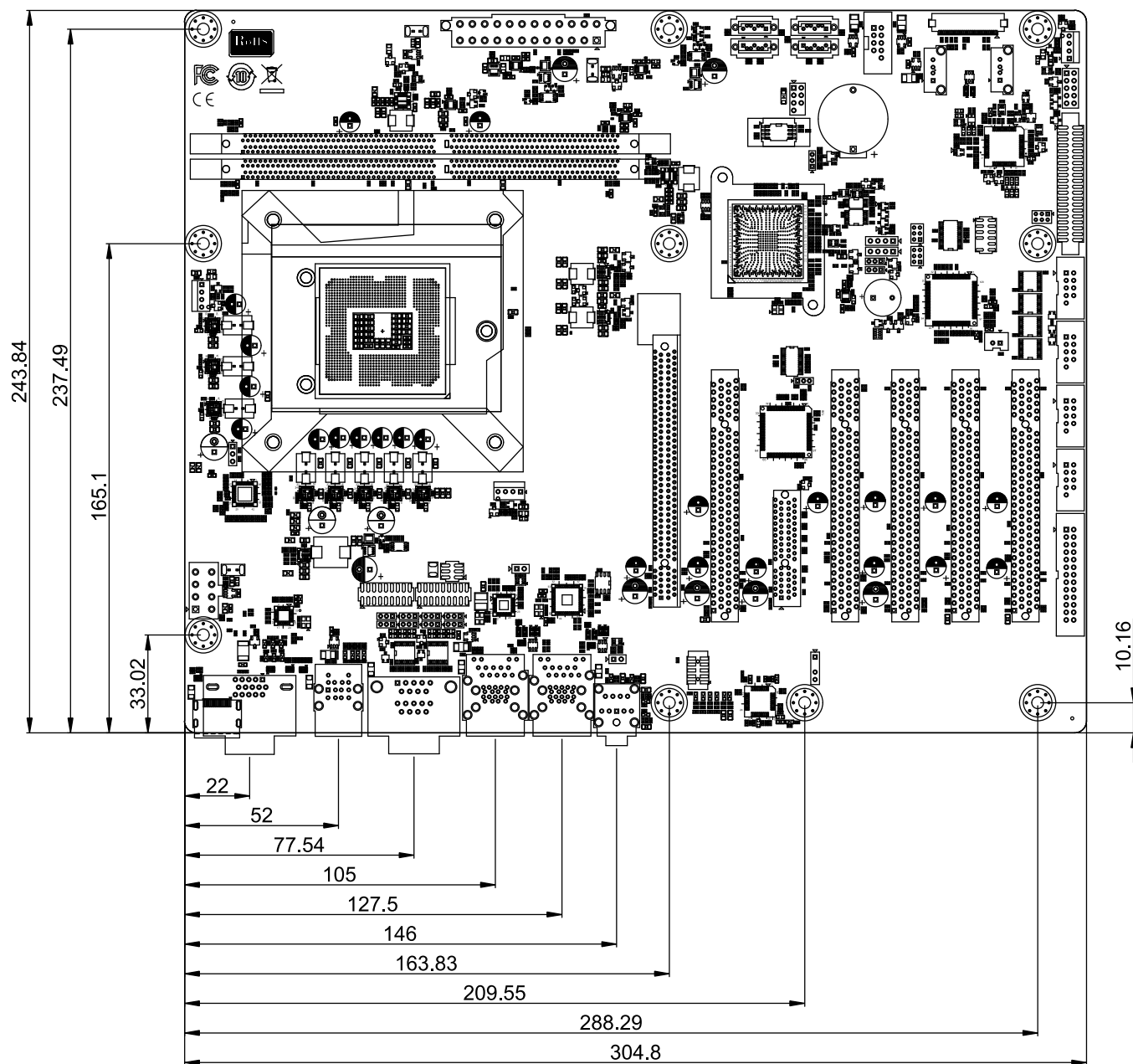
Figure 4: Mechanical Dimensions
