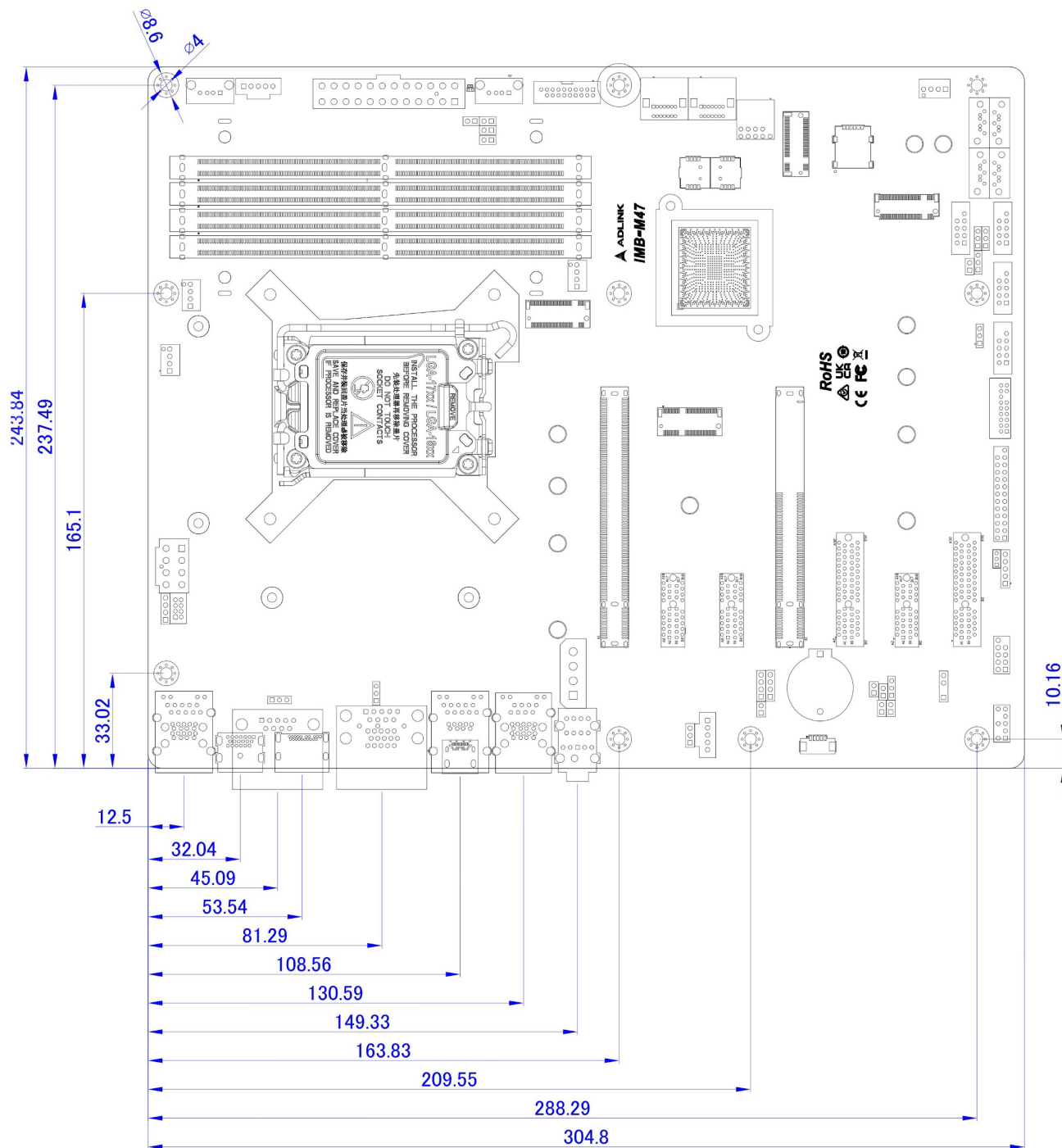
Figure 4: Mechanical Dimensions
