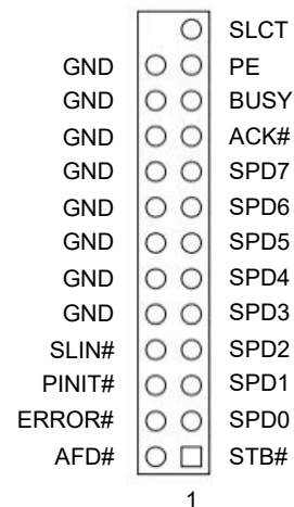
Printer Port
