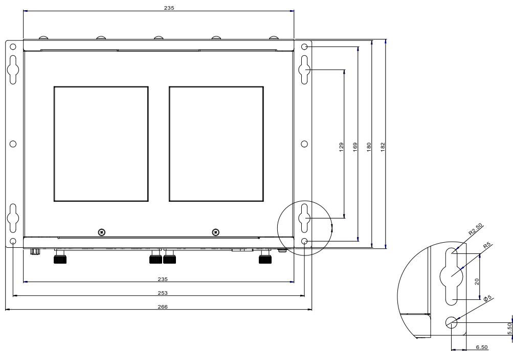
Figure 2-6: MLB-3000 Top View
