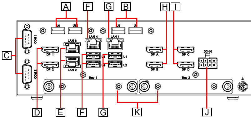
Figure 3-1: MLB-3000 Front Panel I/O
