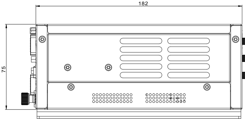
Figure 2-4: MLB-3000 Right Side View
