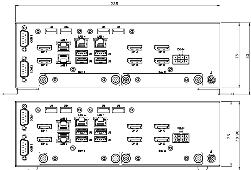
Figure 2-2: MLB-3000 Front View (including wall-mount brackets and footpads)
