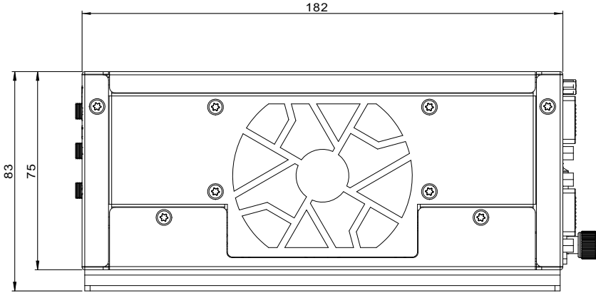
Figure 2-3: MLB-3000 Left Side View
