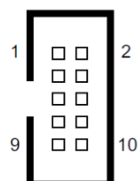
Figure 3-14: COM Connector Pin Definition
