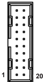
Figure 3-11: USB 3.2 Connector Pin Definition
