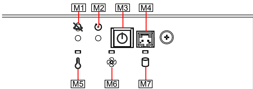
Figure 3-3: Power-on Module
