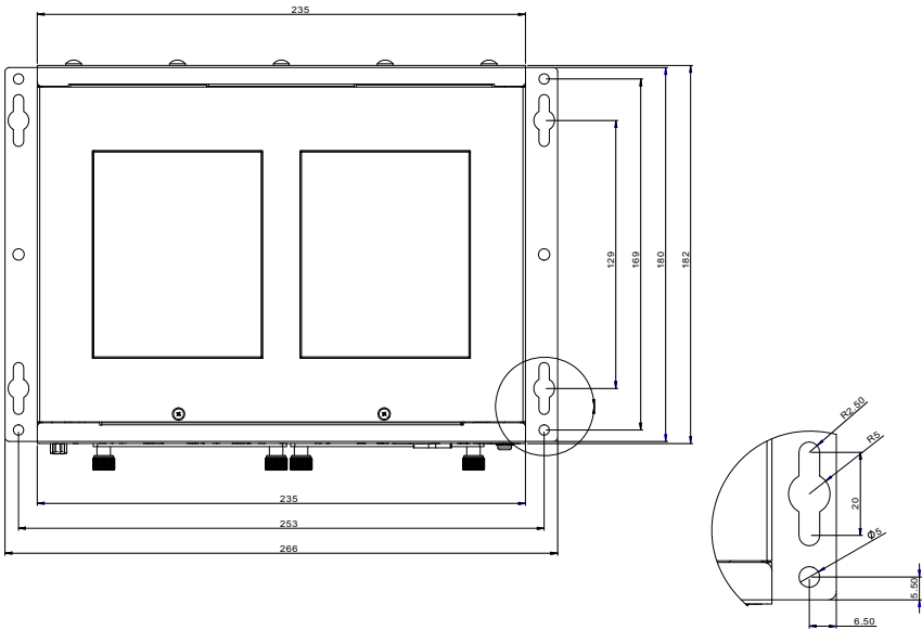
Figure 2-6: MLB-3002 Top View
