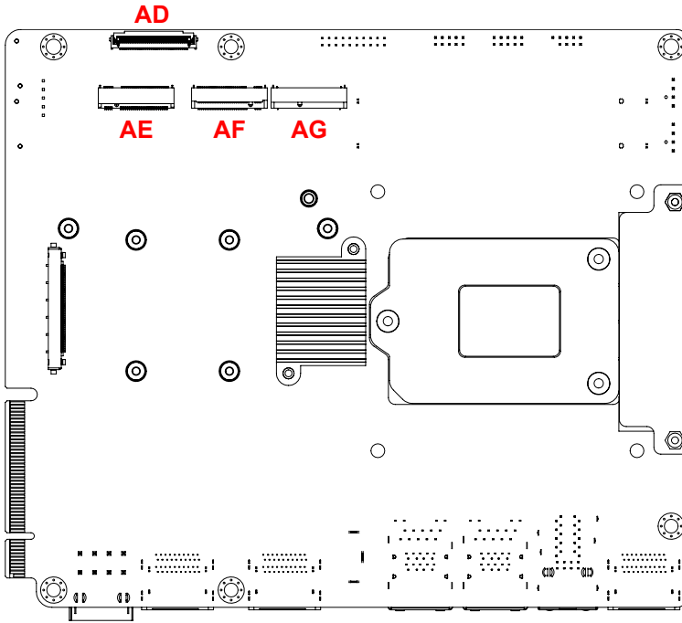
Figure 3-9: Mainboard Connectors (Bottom)
