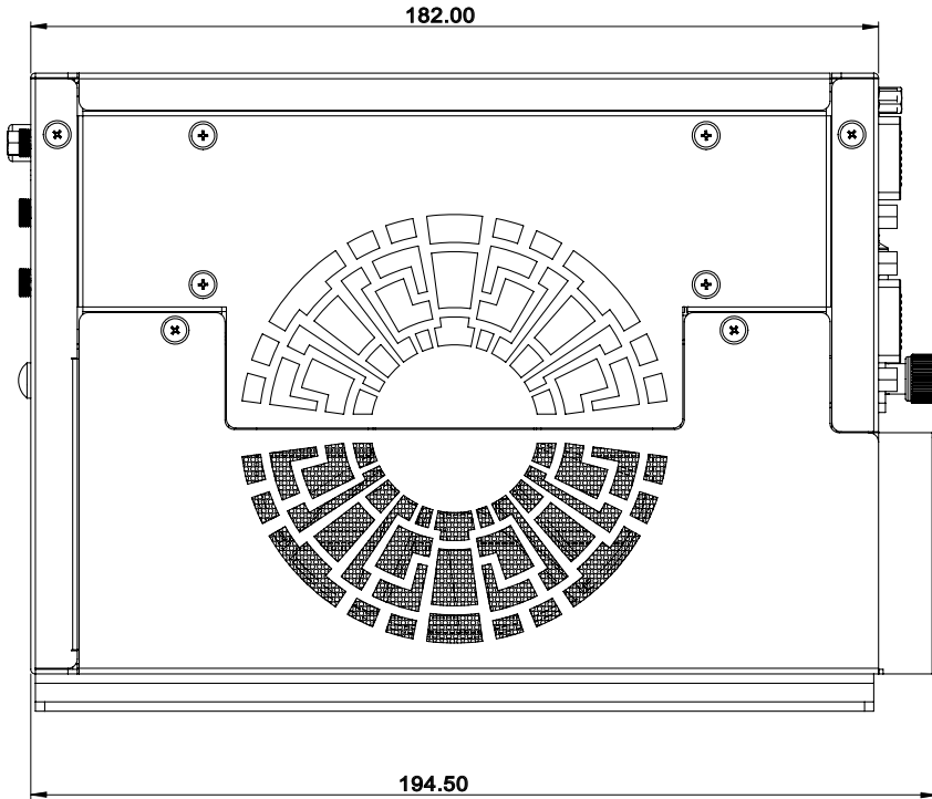
Figure 2-3: MLB-3002 Left Side View
