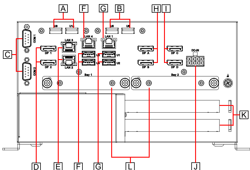
Figure 3-1: MLB-3002 Front Panel I/O
