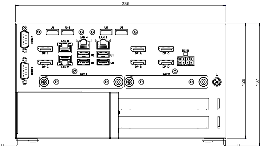
Figure 2-2: MLB-3002 Front View (including wall-mount brackets and footpads)
