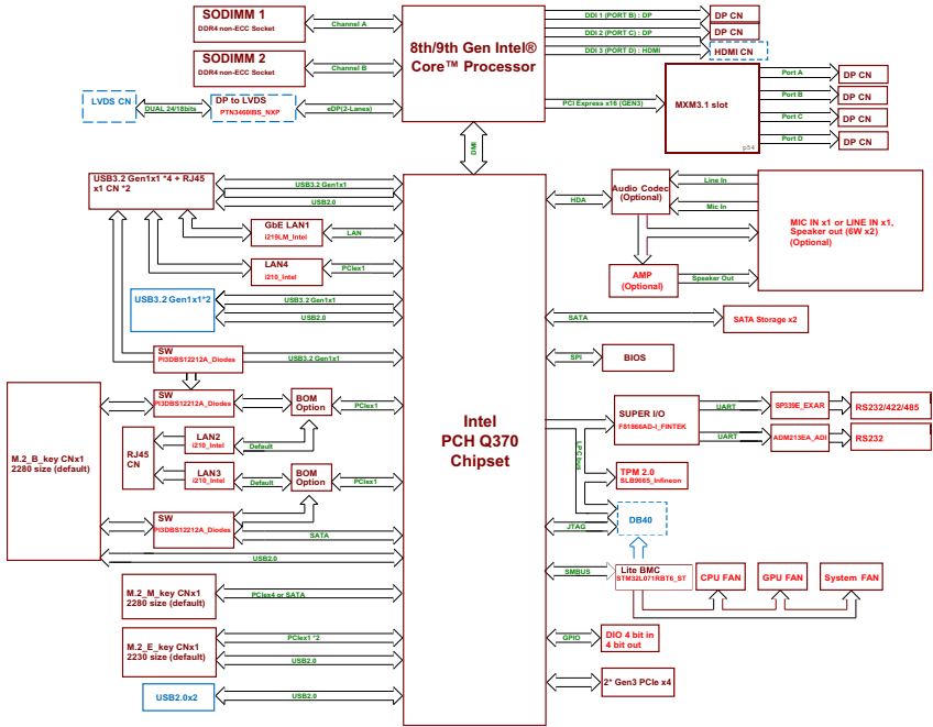
Figure 2-1: MLB-3002 Functional Block Diagram
