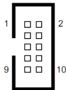
Figure 3-14: COM Connector Pin Definition
