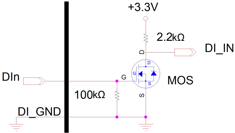
Figure 3-5: Digital Input Circuit
