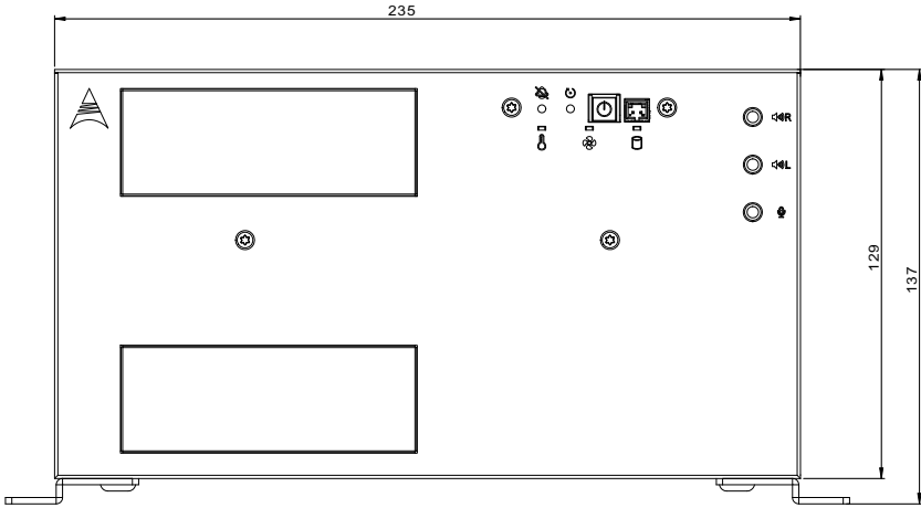
Figure 2-5: MLB-3002 Rear View
