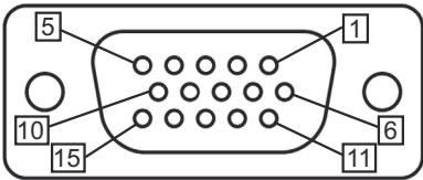
Figure 3-4: Digital I/O Connector Pin Definition
