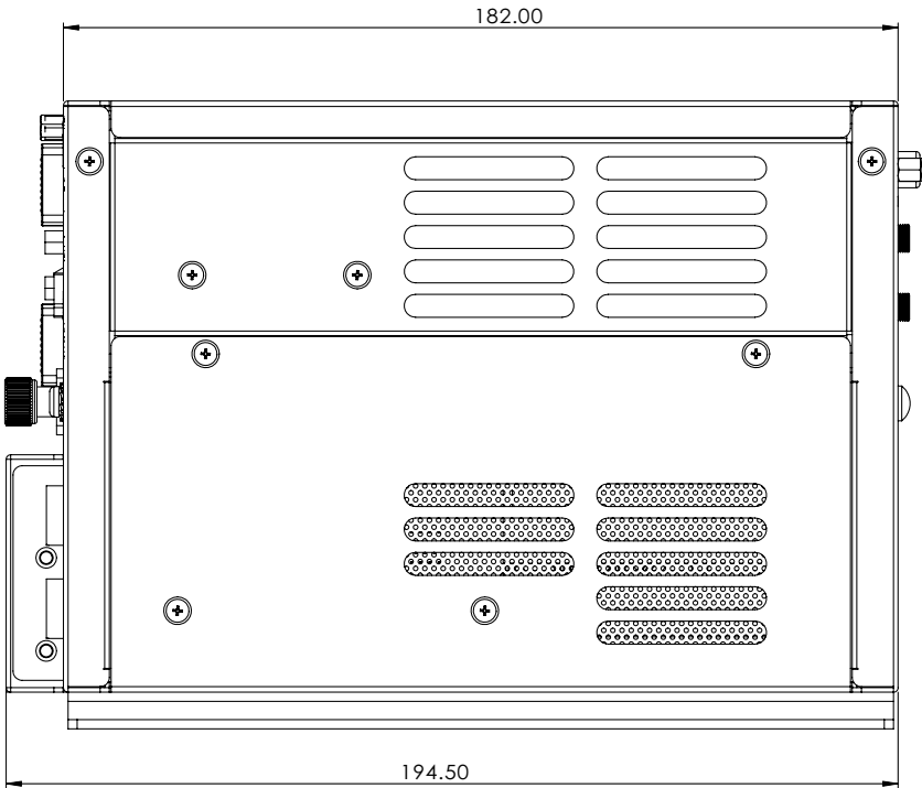
Figure 2-4: MLB-3002 Right Side View
