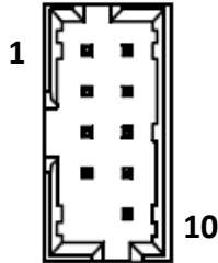
Figure 3-10: USB 2.0 Connector Pin Definition
