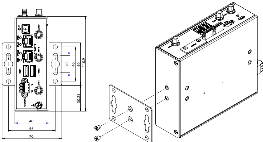
Figure 1-6: Wall Mount 2
