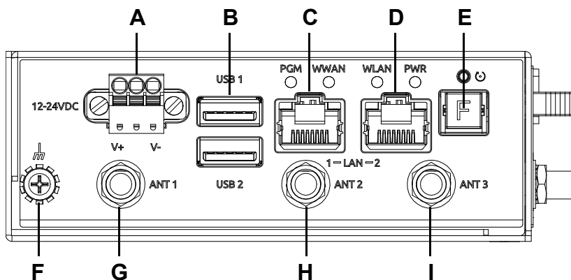
Figure 1-8: Front View
