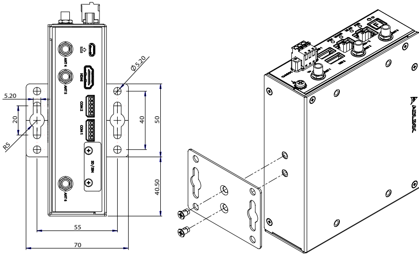
Figure 1-5: Wall Mount 1
