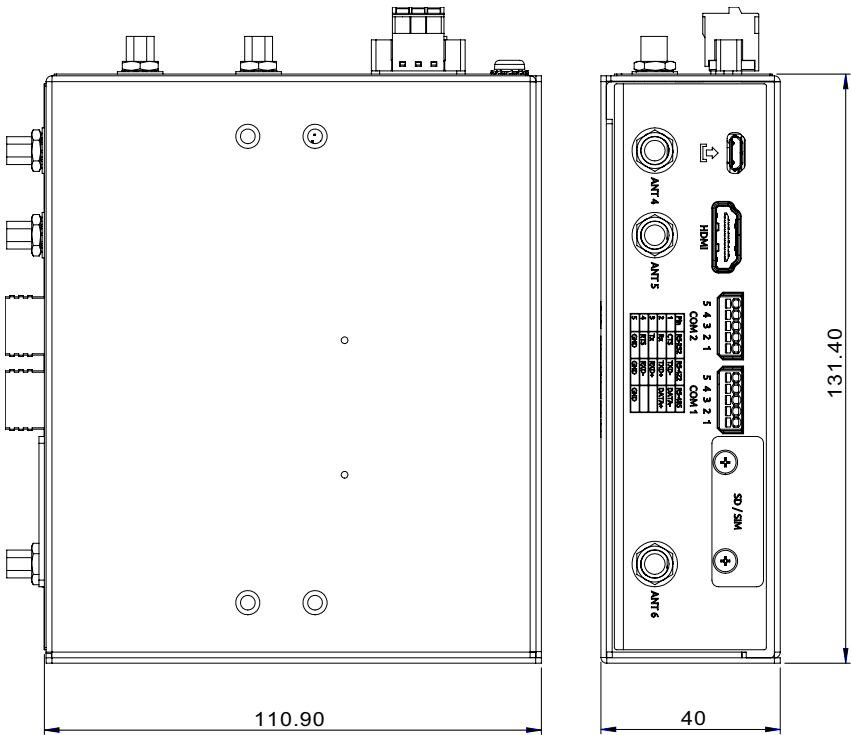
Figure 1-2: MXA-200 Dimensions
