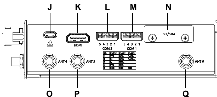
Figure 1-9: Side View
