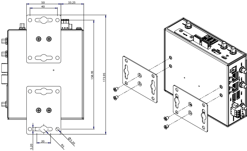
Figure 1-7: Wall Mount 3
