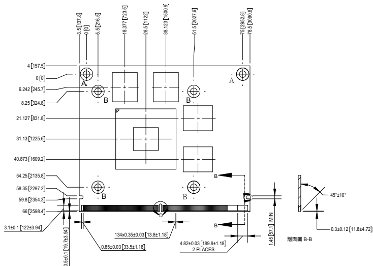
Figure 1-2: MXM-P1000 Component Layout
