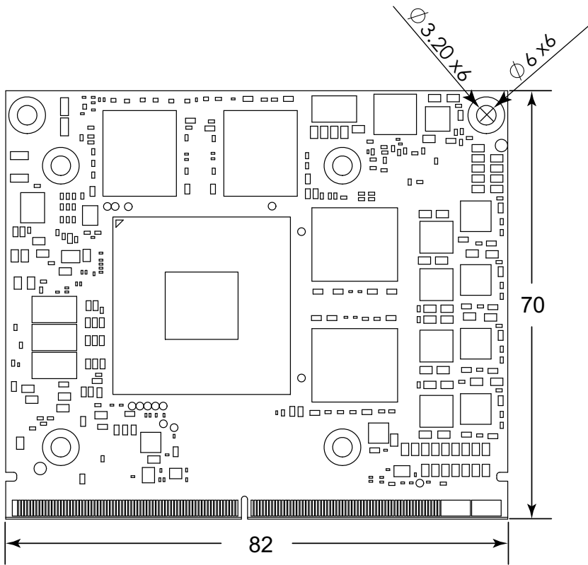
Figure 1-1: MXM-P1000 Dimensions
