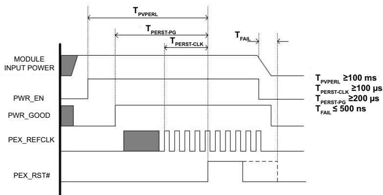
Figure 2-3: Reset Sequencing
