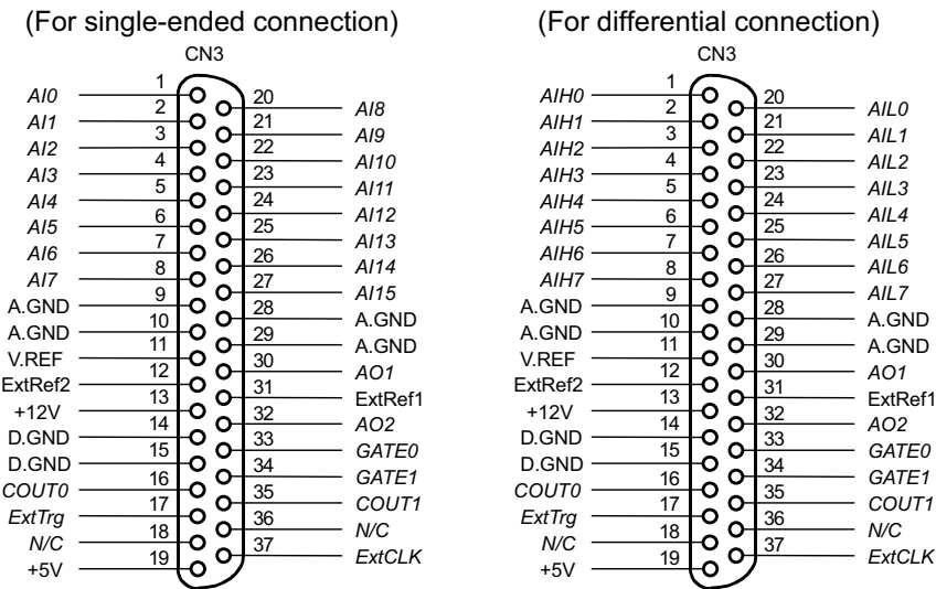
Figure 2-13: PCle-9101 CN3 Pin Assignments
