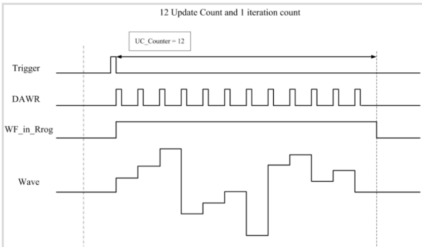
Figure 3-21: Post-Trigger Generation
