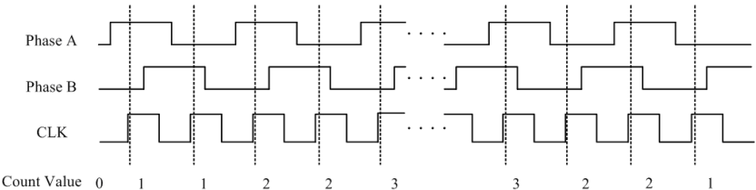
Figure 3-44: X1 Encoder Mode
