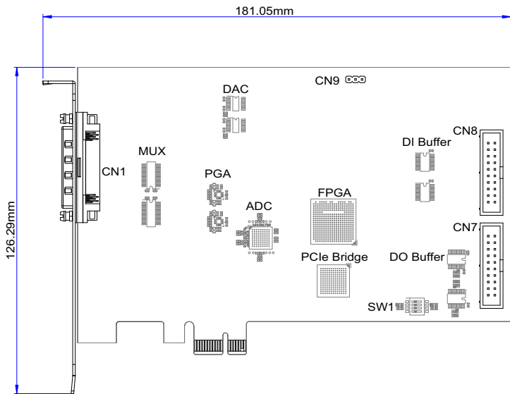
Figure 2-6: PCIe-9161/9163 PCB Front Layout
