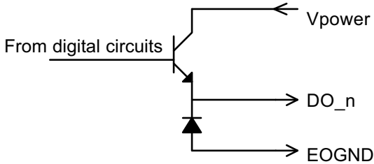
Figure 3-29: Digital Output Circuits
