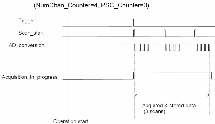
Figure 4-7: Post trigger
