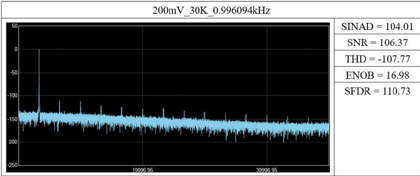
Figure 1-2: Spectral Response (At 30,000-SPS, Typical, 25°C)
