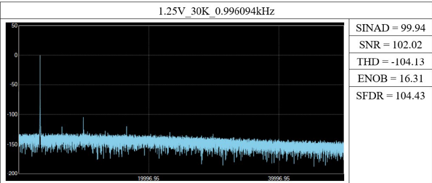
Figure 1-6: Spectral Response ±1.25 V range, 0.996094 Hz sine wave, -1 dB FS
