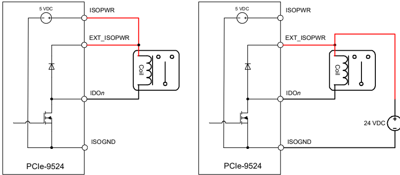
Figure 3-16: Connecting to an external inductive load from an isolated DO sink driver
