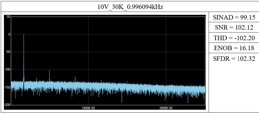
Figure 1-3: Spectral Response \pm 10 V range, 0.996094 Hz sine wave, -1 dB FS
