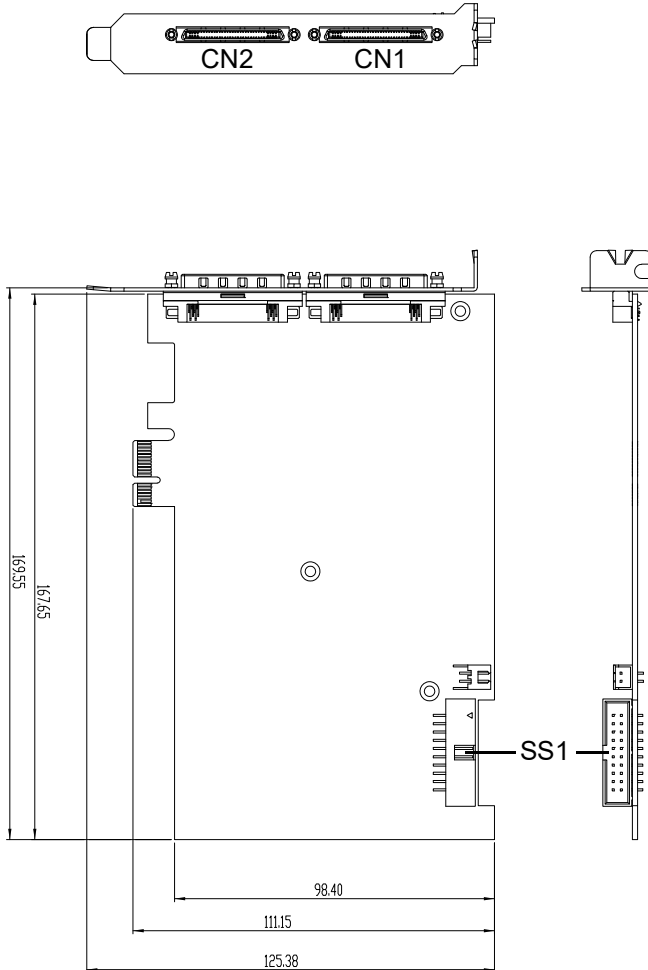
Figure 2-1: PCIe-9524 PCB Layout and Mechanical Drawing
