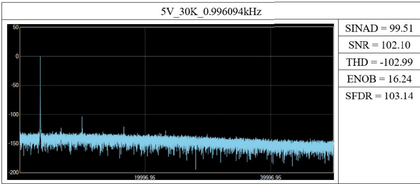
Figure 1-4: Spectral Response \pm 5 V range, 0.996094 Hz sine wave, -1 dB FS
