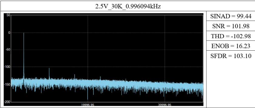
Figure 1-5: Spectral Response ±2.5 V range, 0.996094 Hz sine wave, -1 dB FS
