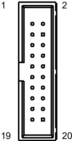
Figure 3-3: SSI Connector & Pin Assignments
