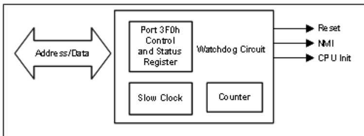
Figure 5-2: W83267HF Watchdog Timer Architecture
