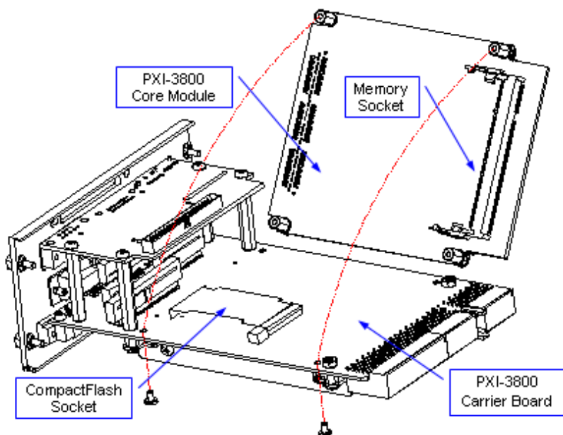
Figure 3-3: Second Memory Module Installation
