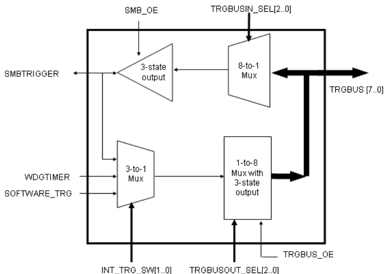
Figure 1-2: PXI Trigger I/O Block diagram
