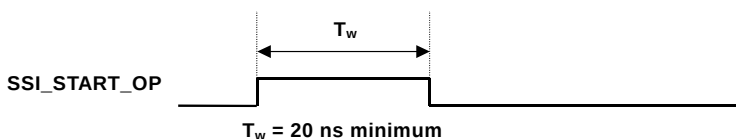
Figure 3.23 SSI_START_OP input signal timing
