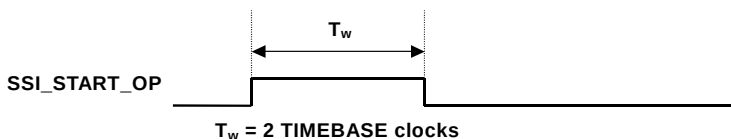
Figure 3.22 SSI_START_OP output signal timing
