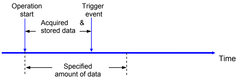
Figure 3.10 Pre trigger (The trigger signal is accepted anytime after the operation starts)
