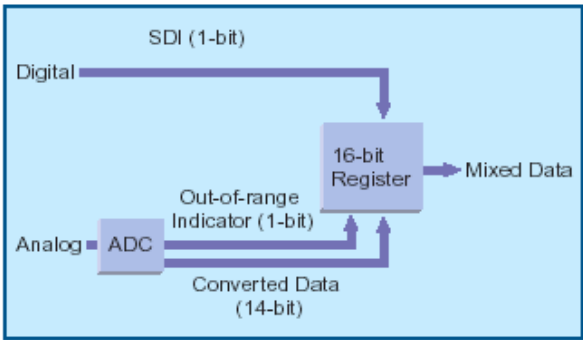
Figure 1.4 PXI-9820 Synchronous Digital Inputs
