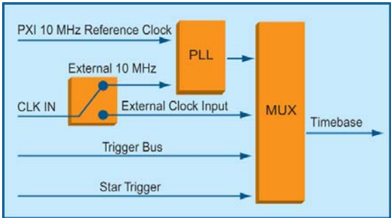
Figure 1.3 PXI-9820 Timebase Control
