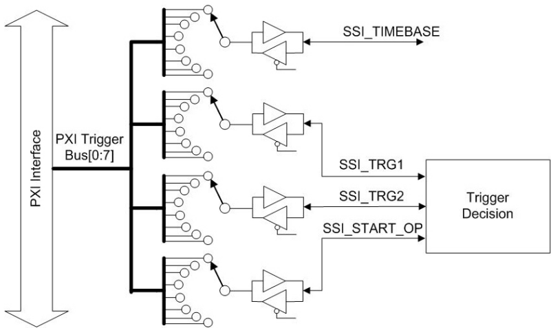
Figure 3.17 SSI Architecture
