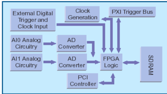
Figure 1.1 PXI-9820 Functional Block Diagram
