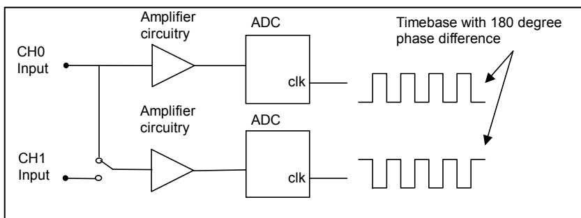
Figure 3.3 “Ping-pong” mode operations
