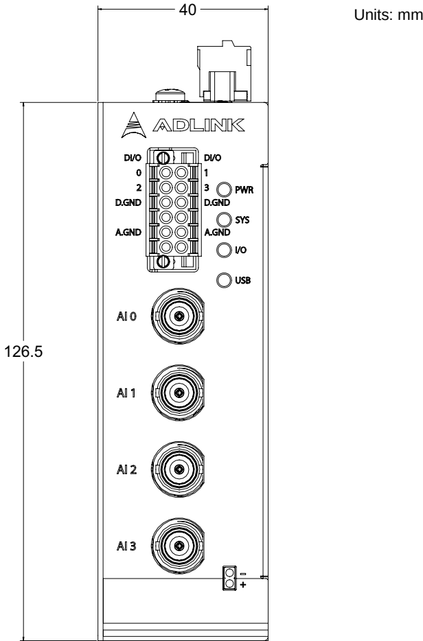
Figure 1-1: Front View
