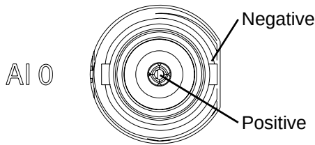
Figure 1-8: BNC Connector Polarity
