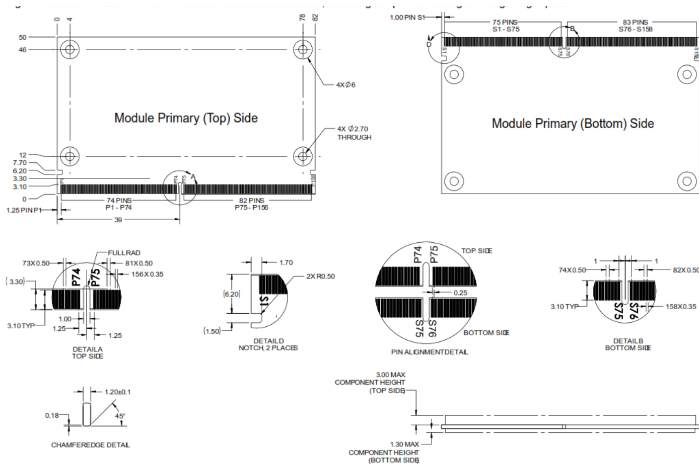
Figure 3 – Mechanical dimensions
