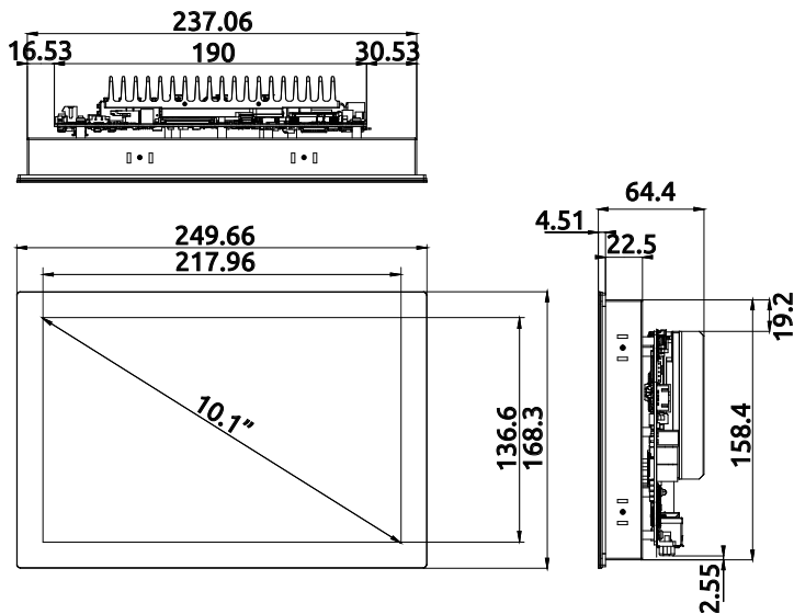
Figure 2-2: SP2-10WP-KL Dimensions
