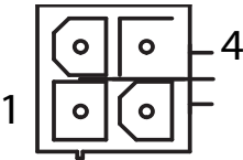
Figure 3-10: Power Connector Pin Definition
