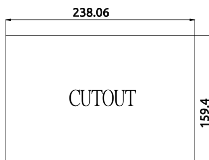
Figure 2-8: SP2-10WP-KL Cutout Dimensions
