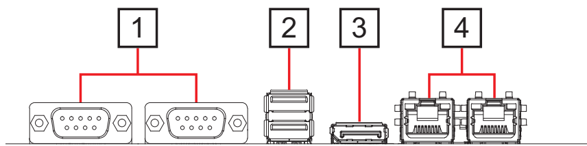
Figure 3-1: SP2-KL Series External I/O
