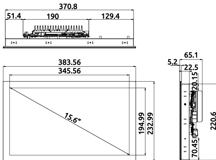
Figure 2-3: SP2-15WP-KL Dimensions
