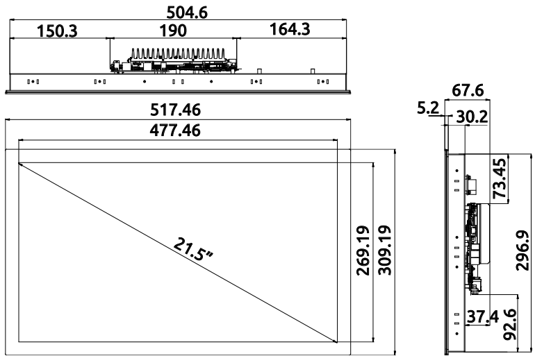
Figure 2-4: SP2-21WP-KL Dimensions
