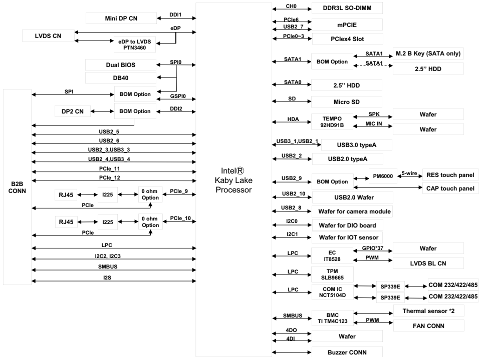
Figure 2-1: SP2-KL Series Block Diagram
