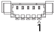
Figure 3-19: Power/Reset Button Connector Pin Definition
