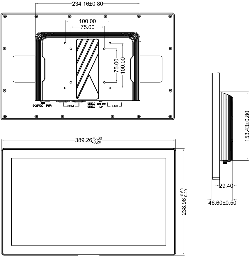
Figure 2-2: STC2-15WP-AL/KL Dimensions
