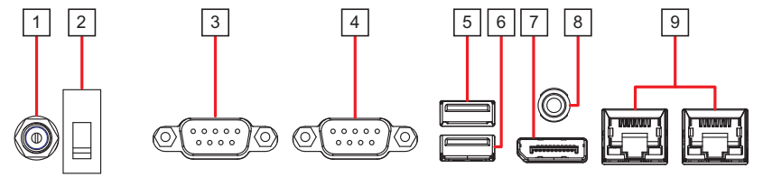
Figure 3-1: STC2-AL/KL Series External I/O (10WP/15WP)
