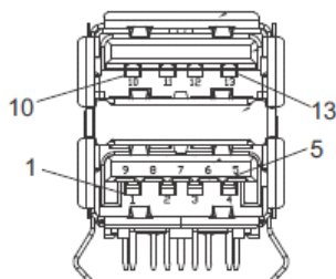
Figure 3-6: USB 3.0 + USB 2.0 Connector Pin Definition
