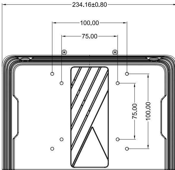
Figure 2-4: STC2-10/15WP-AL/KL VESA mounting
