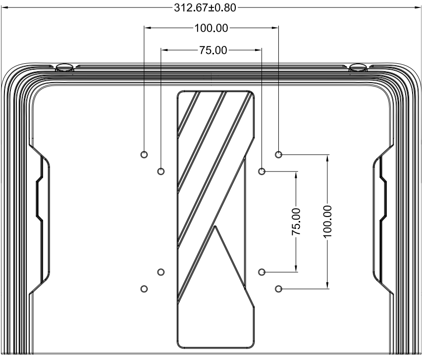
Figure 2-5: STC2-21WP-KL VESA mounting
