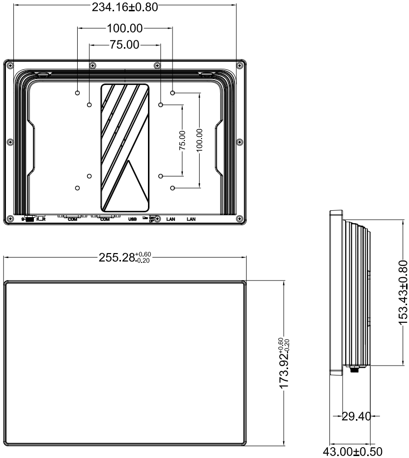
Figure 2-1: STC2-10WP-AL/KL Dimensions
