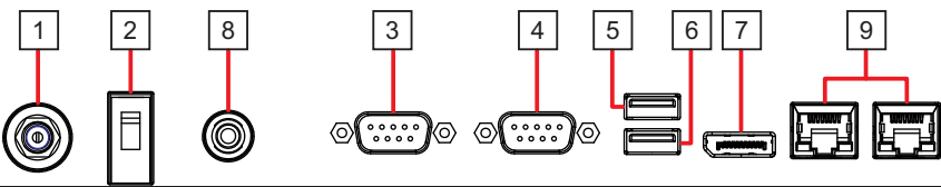
Figure 3-2: STC2-AL/KL Series External I/O (21WP-KL)
